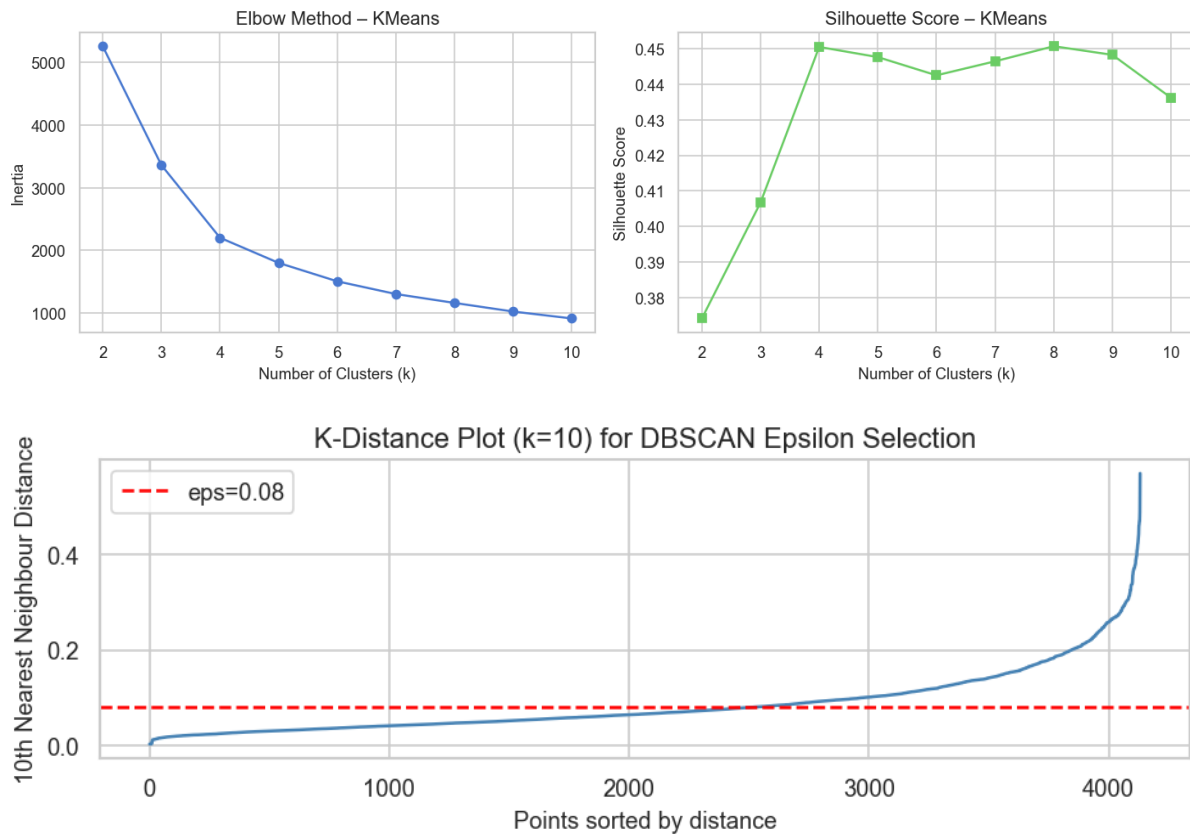
Figure 8: Inertia and Silhouette scores for optimal KMeans cluster selection and K-Distance plot for optimal eps value for DBSCAN
