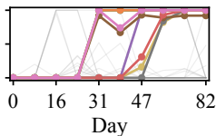
iv Convergent alleles
