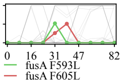
iv Convergent alleles
