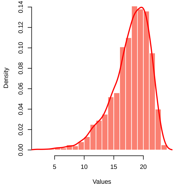
Negatively Skewed
