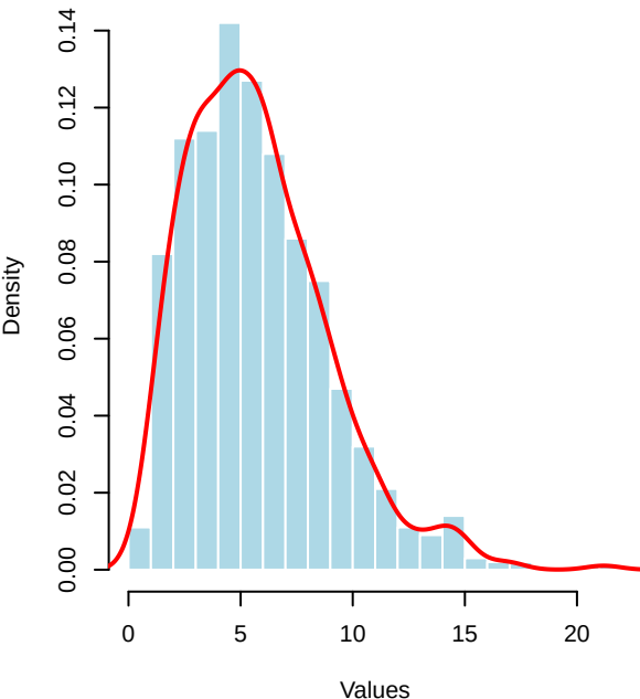
Positively Skewed
