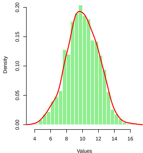
Bell-Shaped (Normal)
