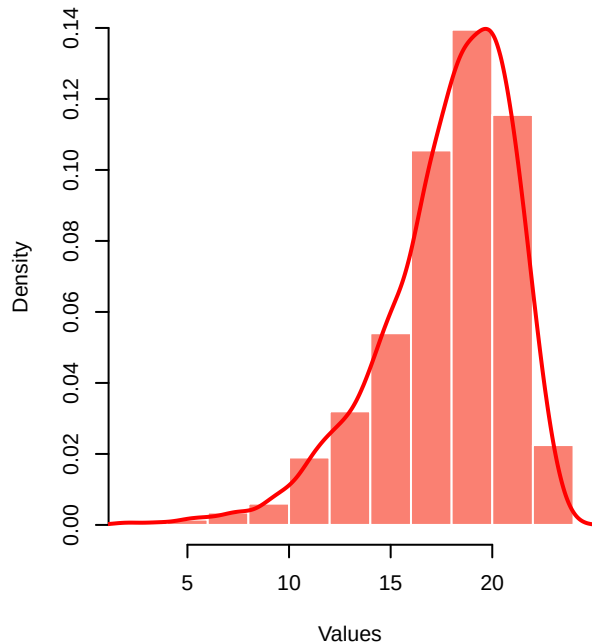
Negatively Skewed
