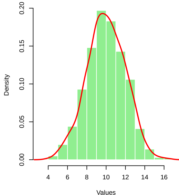
Bell-Shaped (Normal)
