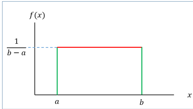
Figure 5.1: Graph of f(x)
