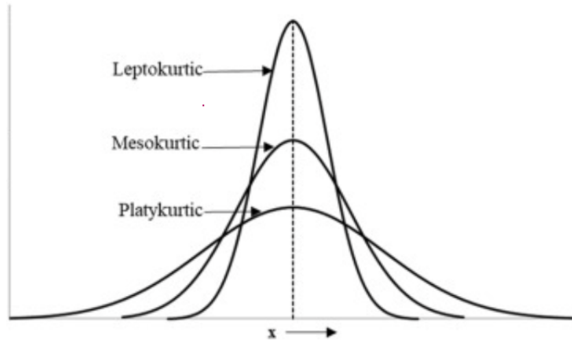
Figure 2.5: Different types of kurtosis
