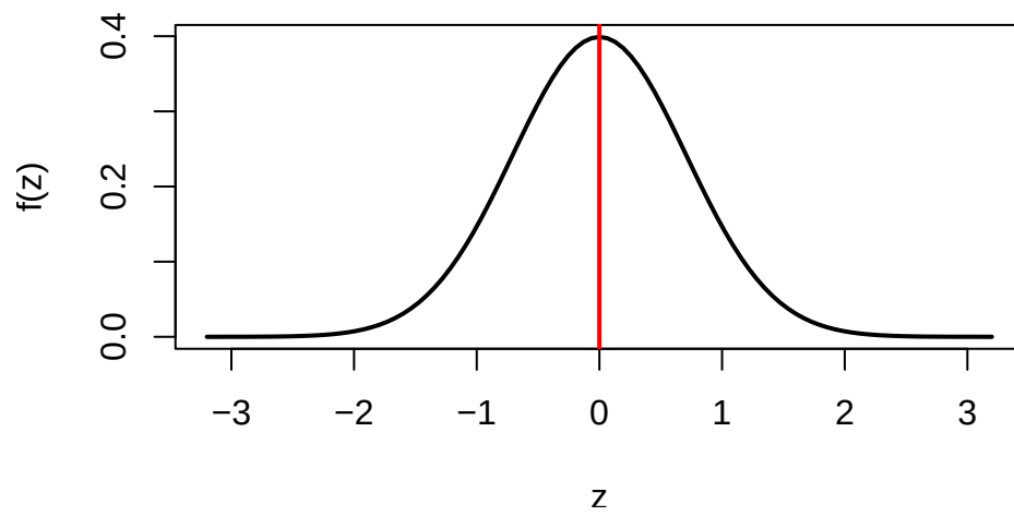
Figure 5.4: Standard normal curve
