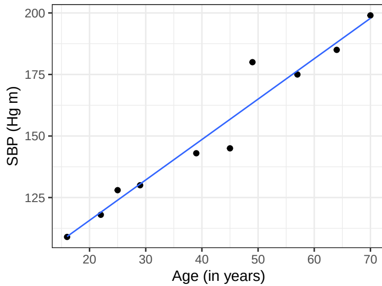
Figure 13.5: Sacter plot of Age and SBP
