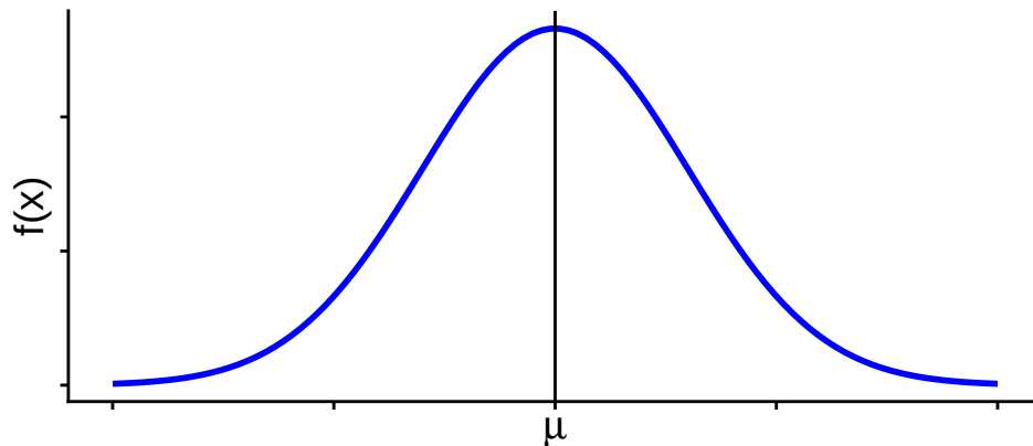
Figure 5.3: Normal Curve
