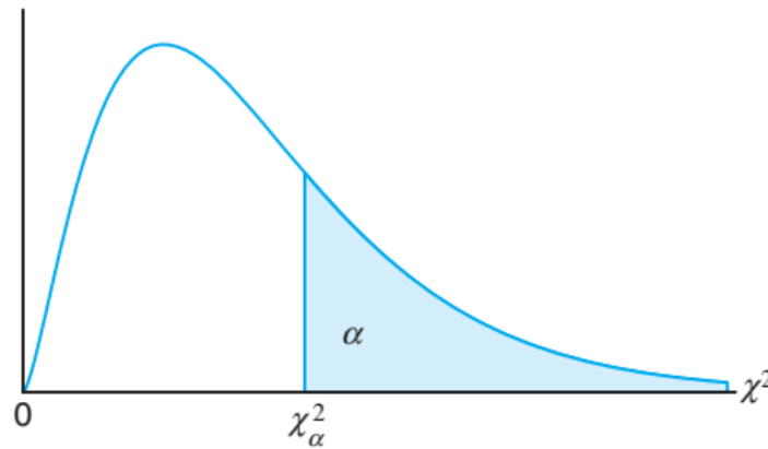
Figure 7.4: The chi-squared distribution
