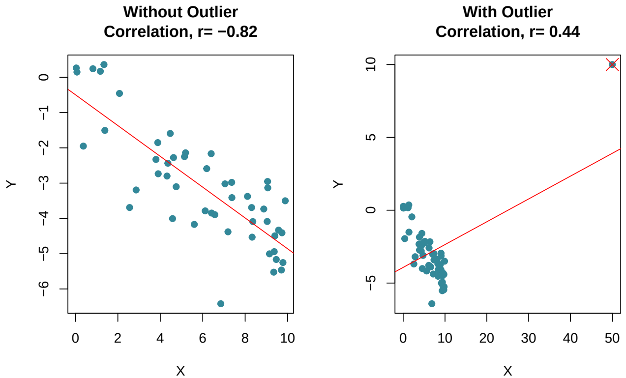
Figure 13.4: Effect of outlier on the sign of correlation coefficient ( r )
