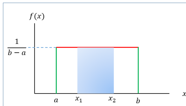
Figure 5.2: Computing area for an interval of Uniform distribution
