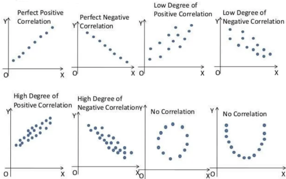
Figure 13.1: Types of correlations that can be represented using a scatter plot
