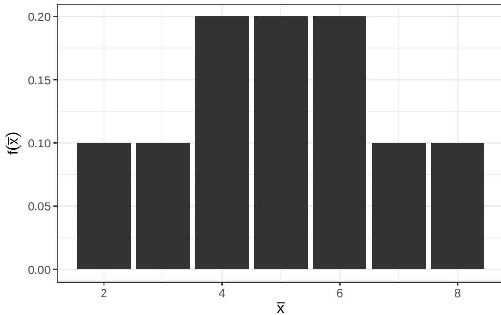
Figure 7.1: Sampling distribution of \bar{x}
