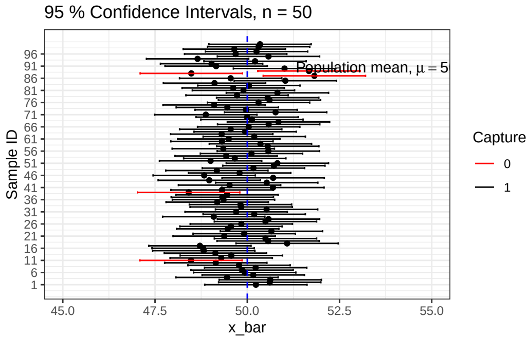
Figure 8.1: Simulation of 95% confidence intervals for \mu
