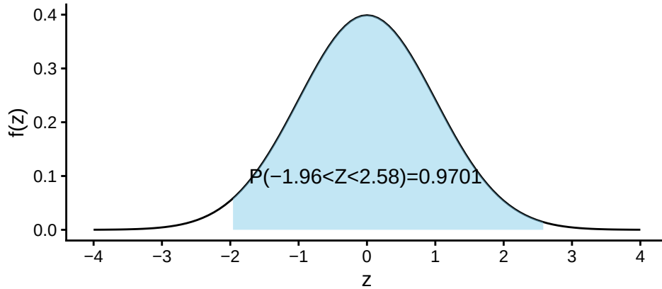
Figure 5.7: Area under standard normal curve for -1.96 < Z < 2.58
