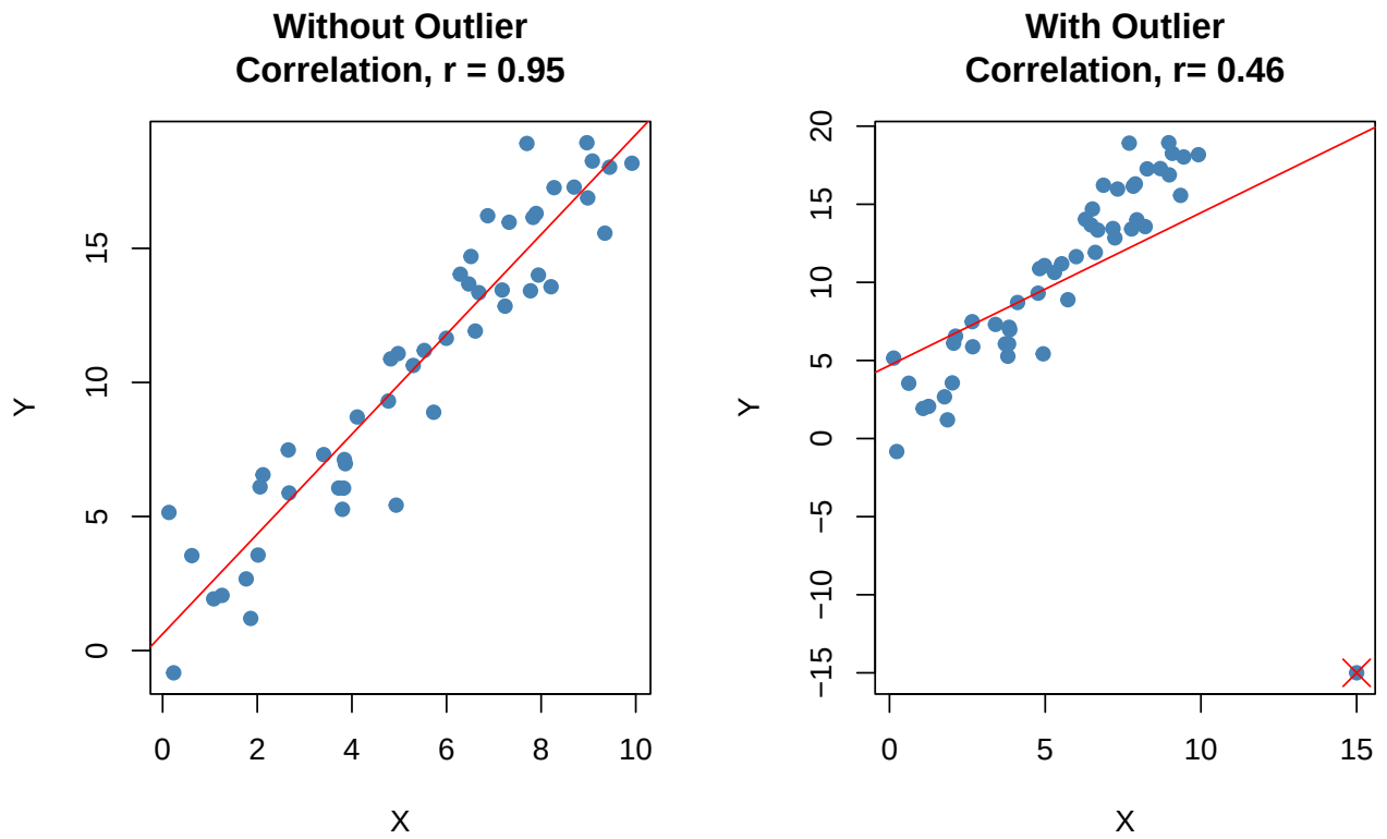
Figure 13.3: Effect of outlier on the magnitude of correlation coefficient ( r )
