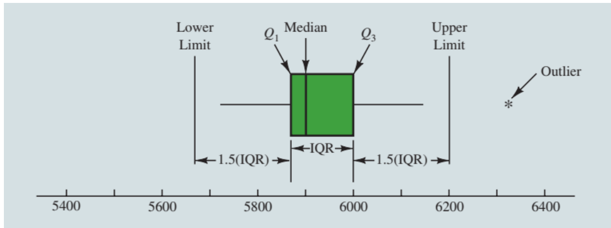
Figure 2.2: Boxplot of the Monthly Starting Salary Data with Lines Showing the Lower and Upper Limits
