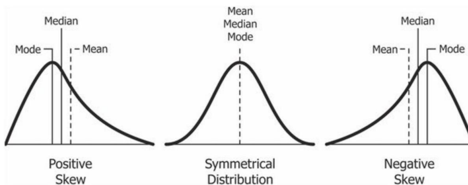
Figure 2.4: Types of skewness and relative position of mean, median, mode
