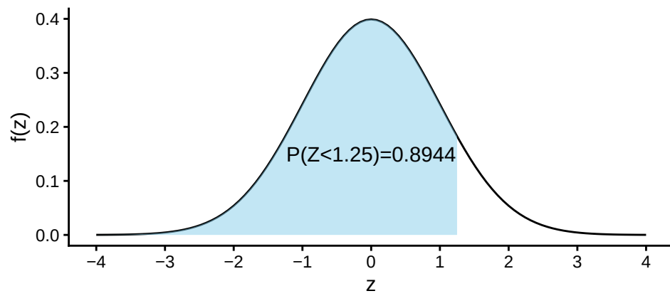
Figure 5.5: Area under standard normal curve for Z < 1.25
