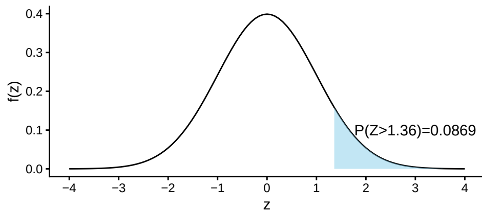
Figure 5.6: Area under standard normal curve for Z > 1.36
