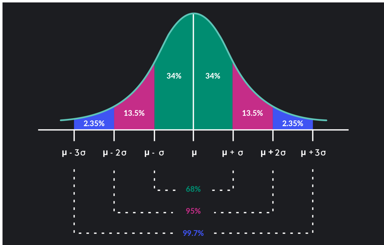
Figure 2.1: Empirical rule
