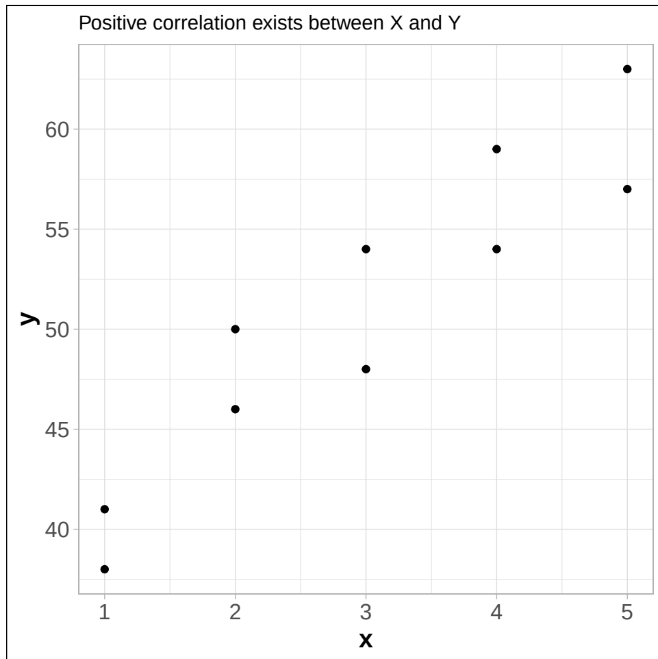
Figure 13.2: Scatter plot between X and Y
