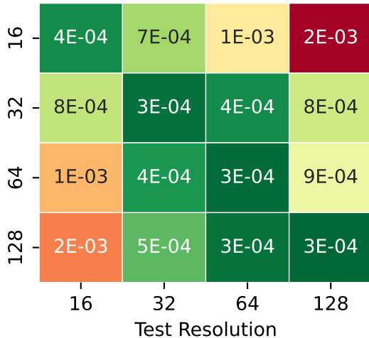
FNO2D
