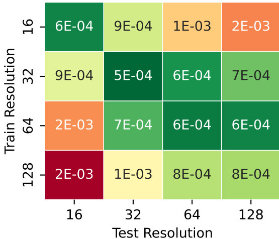
DeepONet2D
