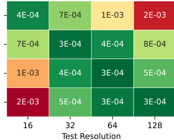
Random Seed: 2
