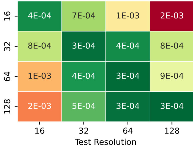
Random Seed: 0
