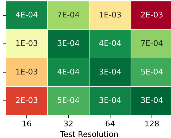
Random Seed: 1
