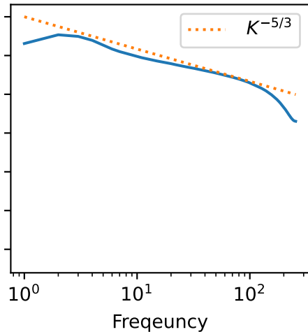
Navier Stokes (2D)
