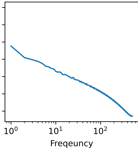
Burgers (1D)
