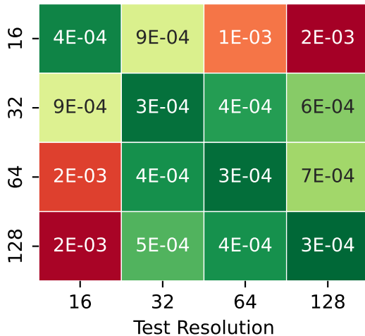
Anti-Alias Activation
