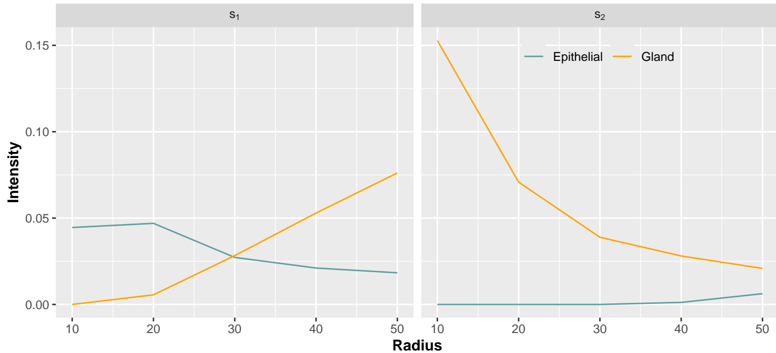
Intensity within circles centered at a fixed location s_l
