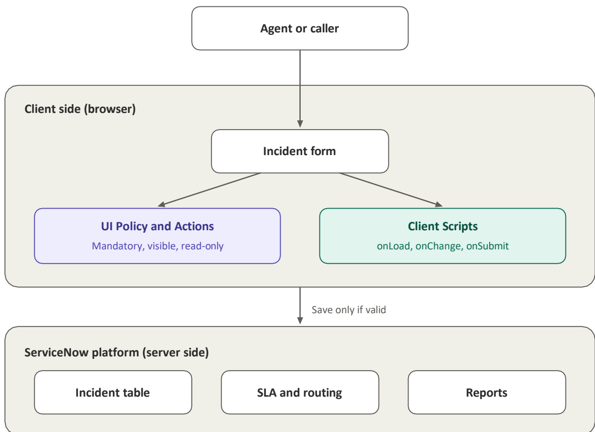
Figure 1: Solution architecture for client-side validation of Incident records
