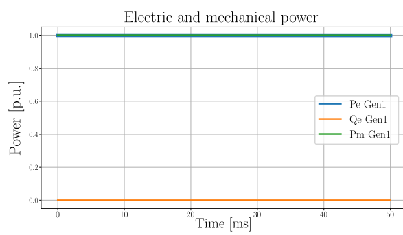
Figure 4.21: Electrical P_e , Q_e and mechanic P_m power of the generator rotor.
