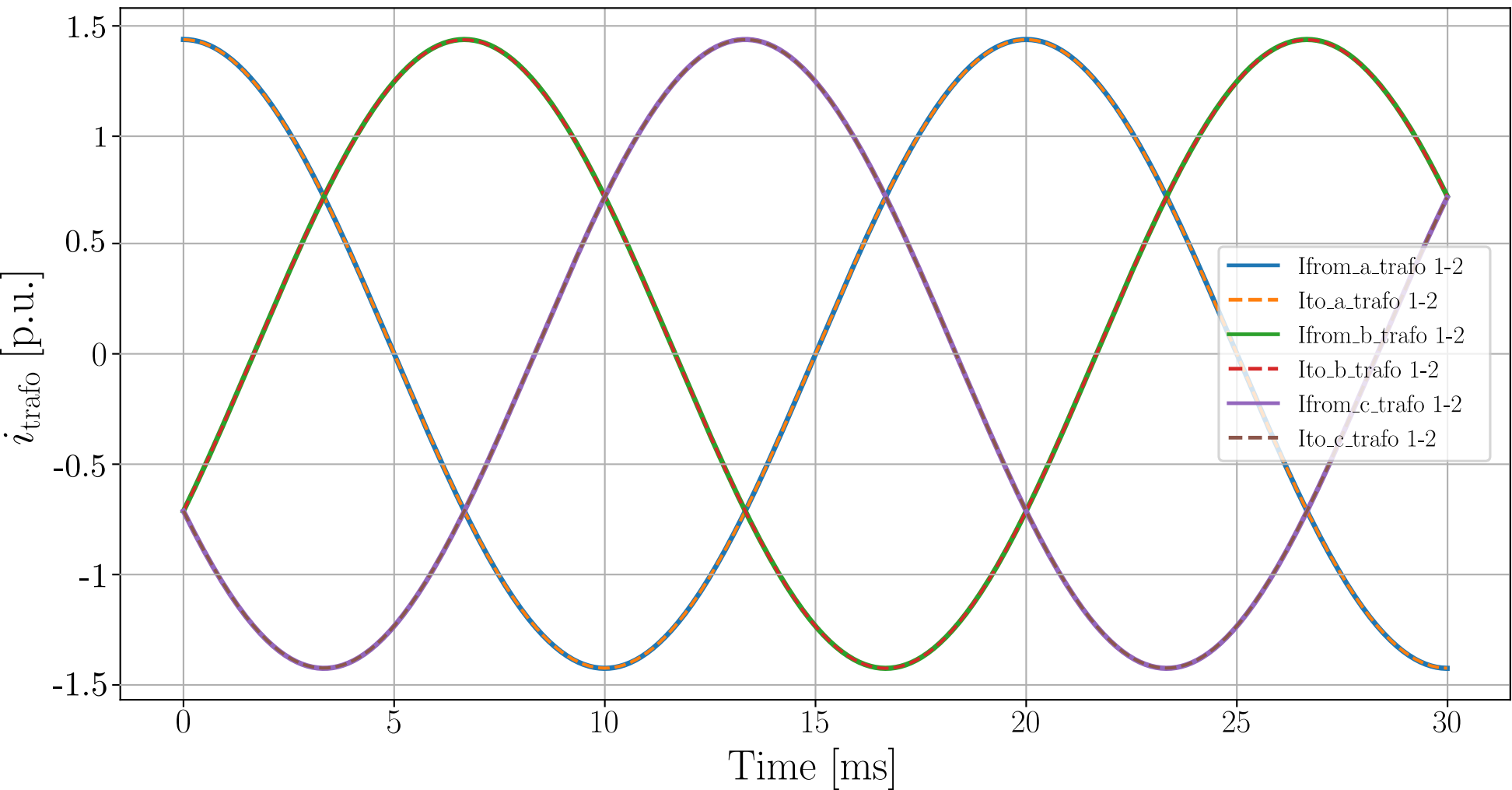
Transformer currents
