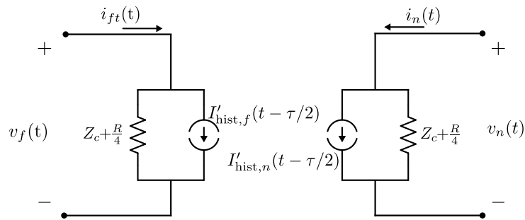
Figure 4.3: Half Bergeron's line model with lumped resistance.
