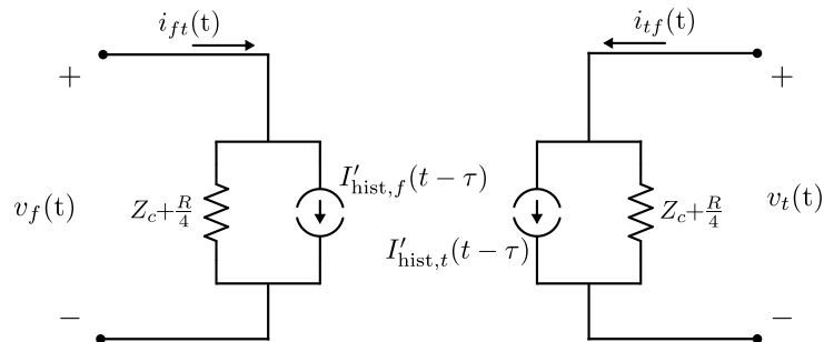
Figure 4.4: Bergeron's line model with lumped resistance two nodes equivalent.
