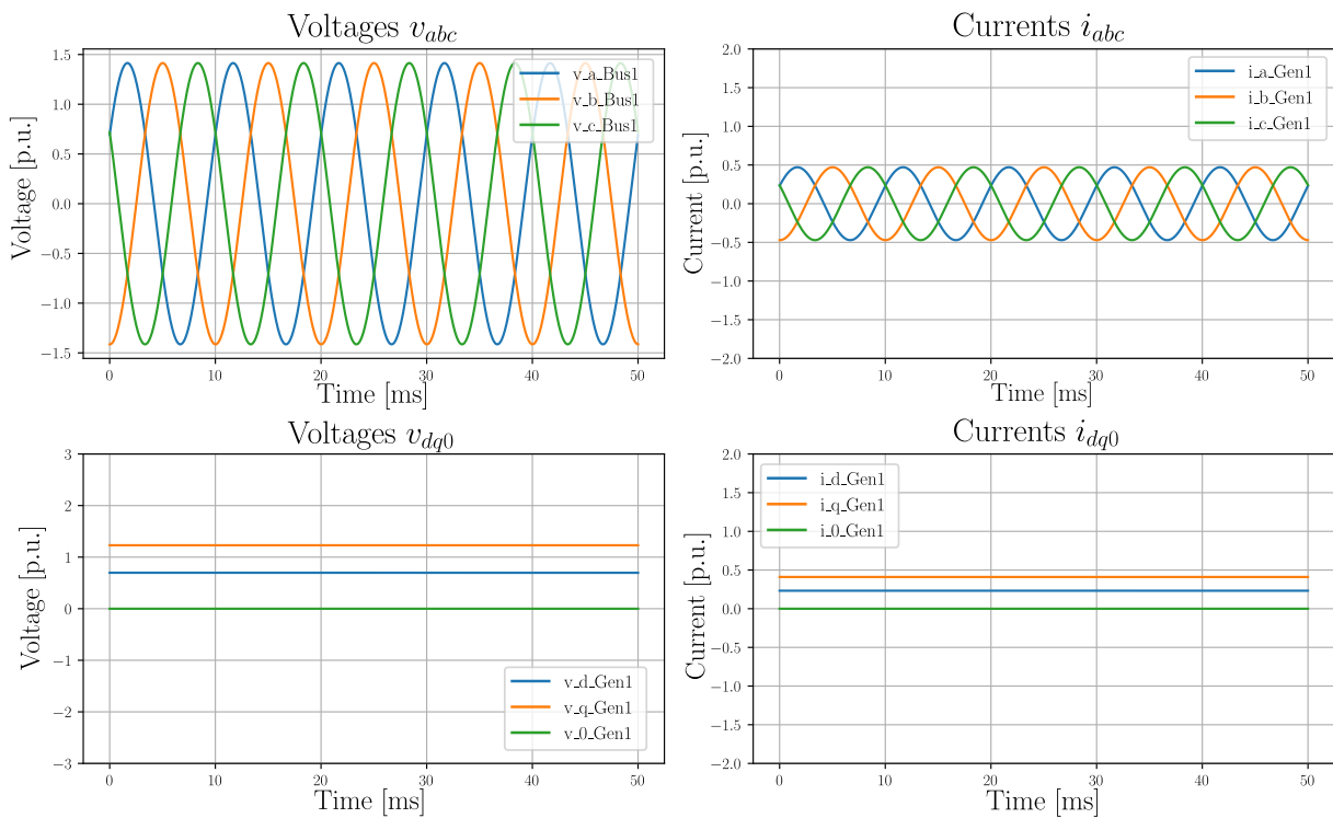
Figure 4.14: Voltages and currents at the 1 bus case.
