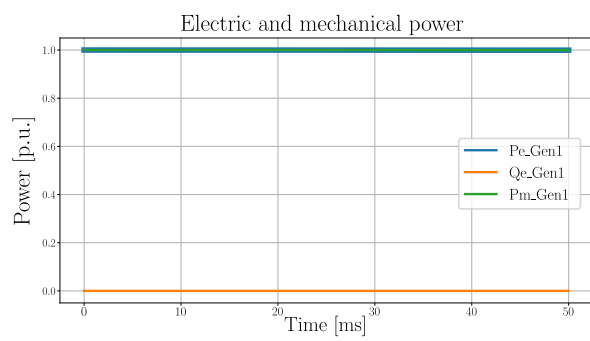
Figure 4.18: Electrical P_e , Q_e and mechanic power P_m of the generator rotor.
