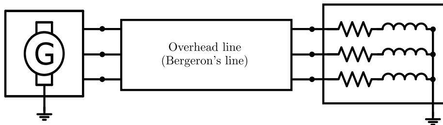
Figure 4.20: Test case 2: Two-bus system diagram.
