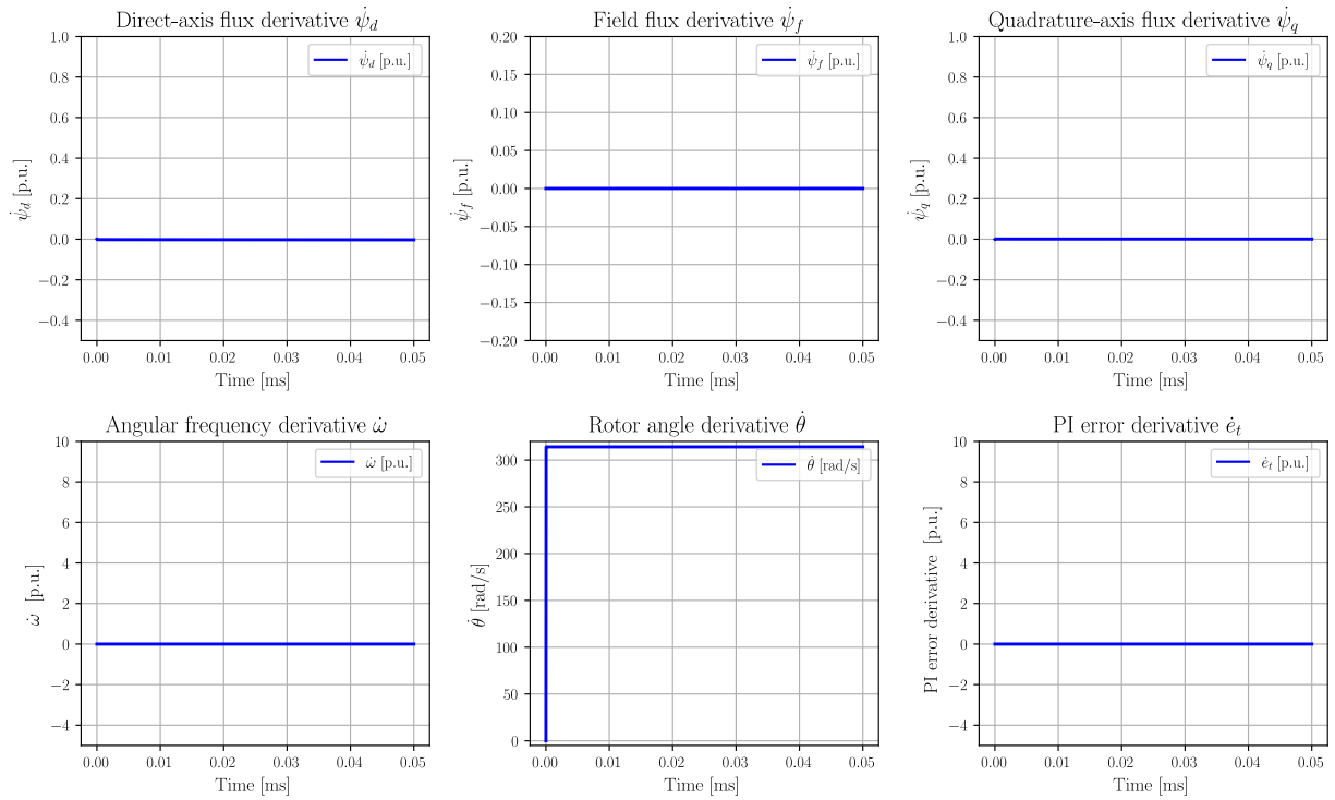
Figure 4.19: Derivatives of state variables at the 1 bus case.
