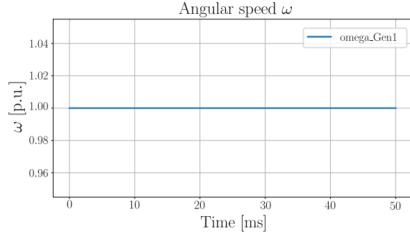
Figure 4.16: Angular speed \omega of the generator rotor.
