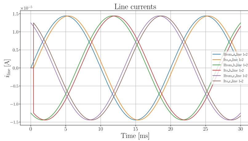
Figure 4.22: Line currents at the 2 bus case. WITH VOLTAGE SOURCE!! TO CHANGE
