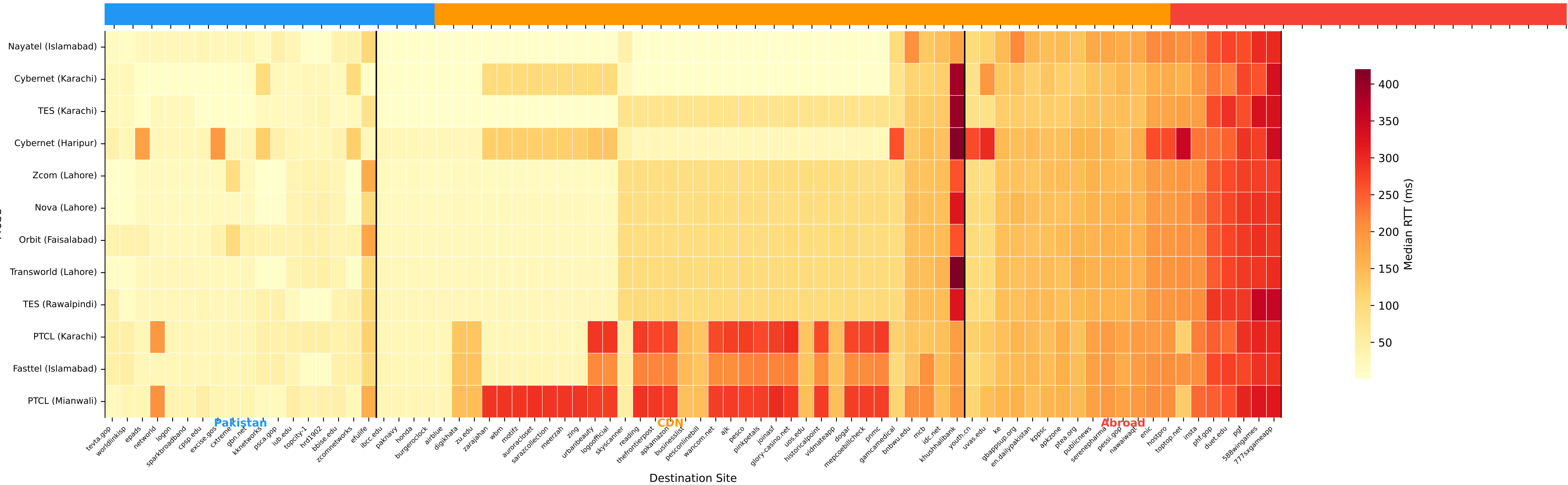
Median Ping RTT (ms) — All Probes × All Sites, Grouped by Hosting Class
