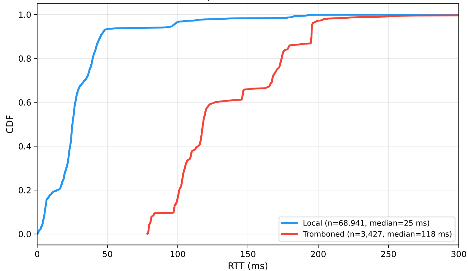
RTT CDF -- Local vs Hairpinned Rounds, PK-hosted Sites (Pooled)
