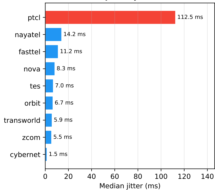
Jitter by ISP
