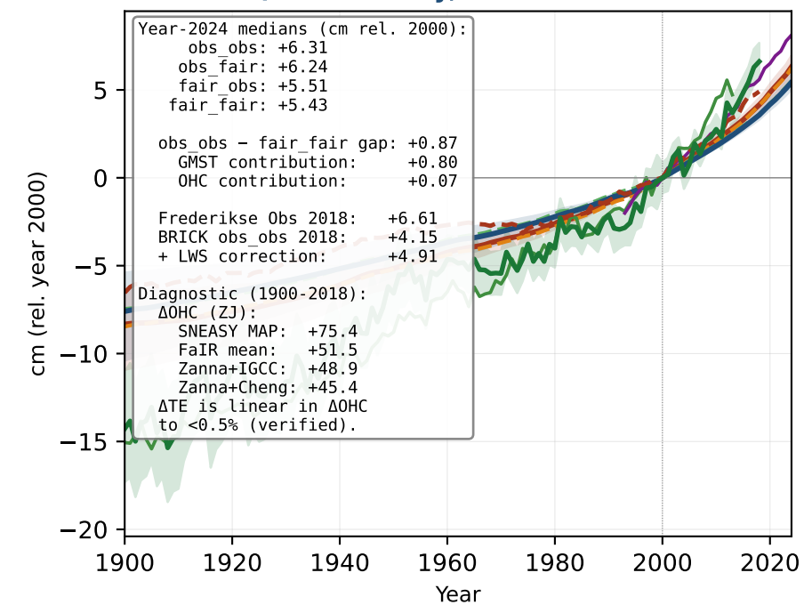
Total GMSL (climate-only, LWS-excluded historical)
