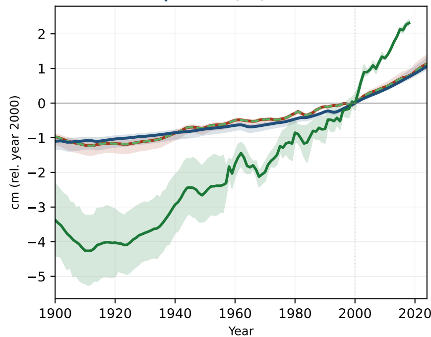
Thermal expansion (TE) — linear in ΔOHC
