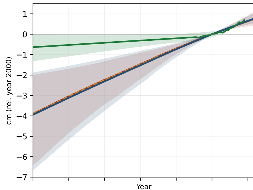
Thermal expansion (TE) — linear in ΔOHC
