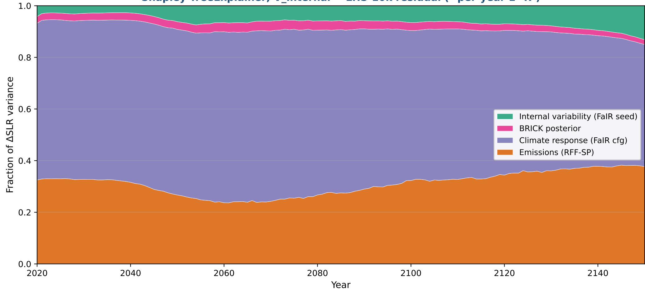
Total \Delta SLR (relative to 2020) Shapley TreeExplainer; V_internal = LHS-10k residual ( \sim per-year 1-R^2 )
