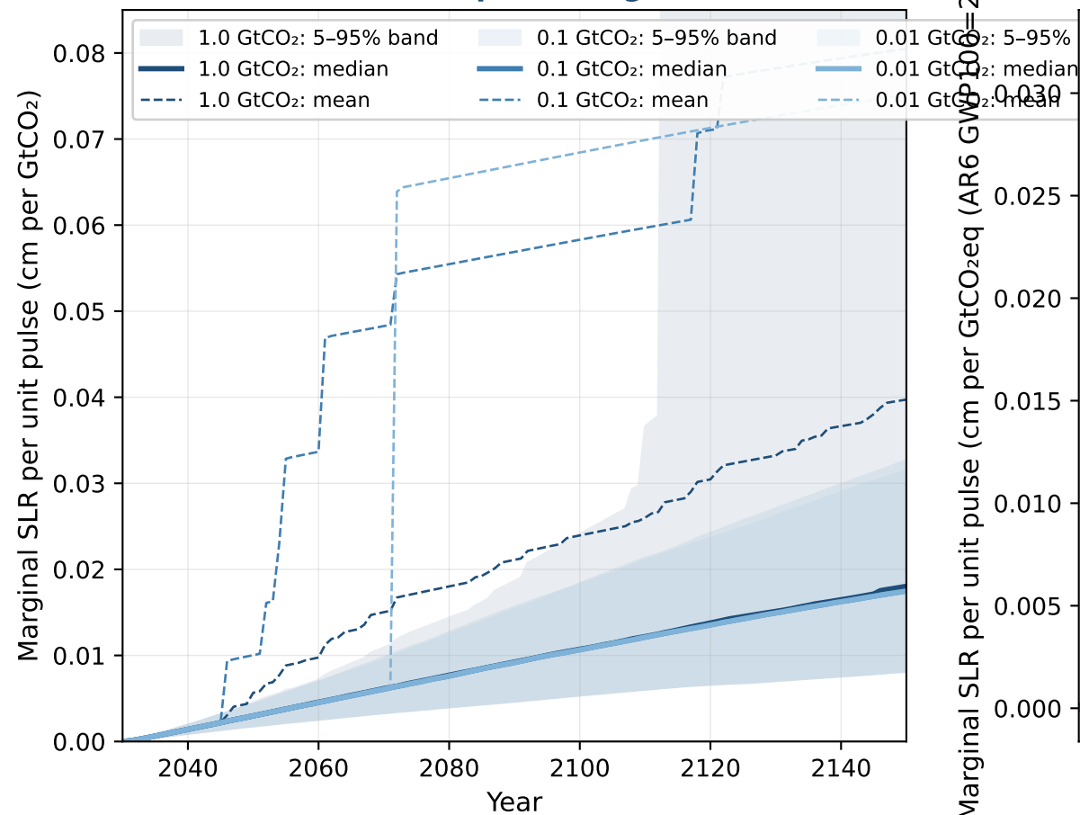
CO2 pulse at 2030 — per-unit marginal SLR vs year across three pulse magnitudes
