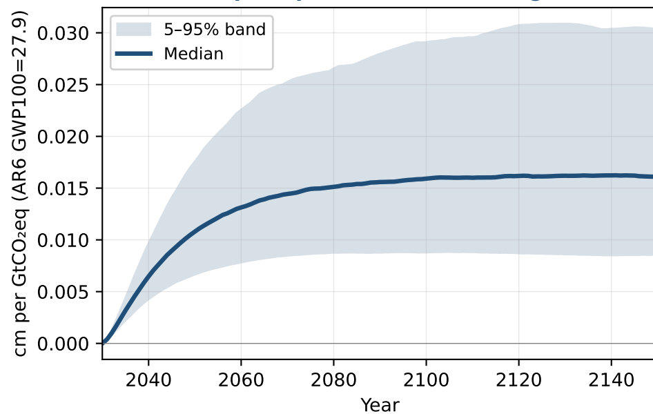
1 GtCO 2 eq CH 4 pulse at 2030 — Marginal SLR
