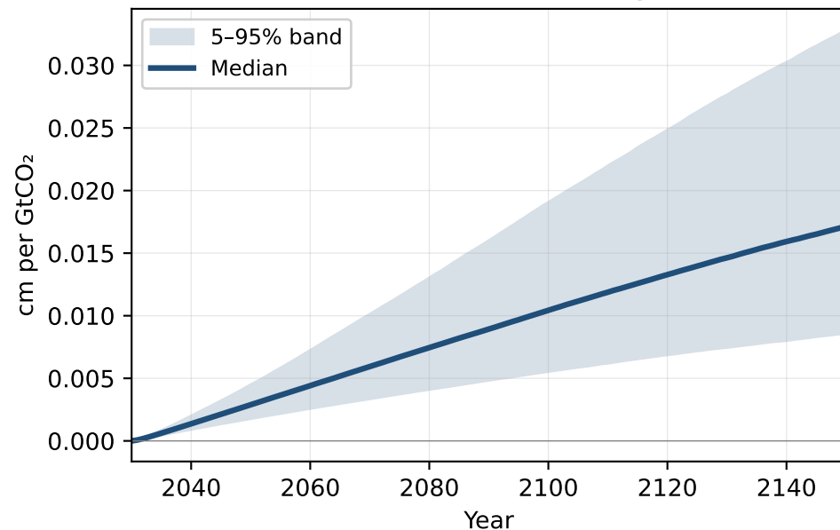
1 GtCO 2 pulse at 2030 — Marginal SLR
