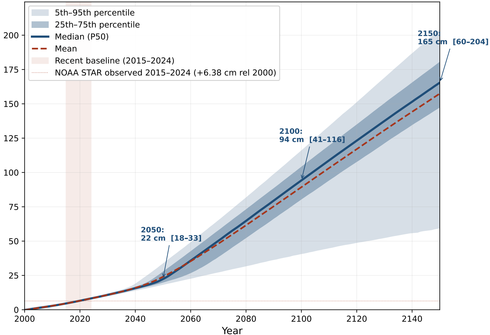
Global Mean Sea Level Rise (cm rel. 2000) AR6-style bias-corrected
