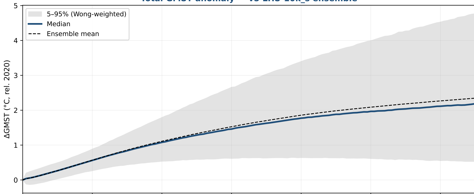
Hawkins-Sutton decomposition — total GMST
