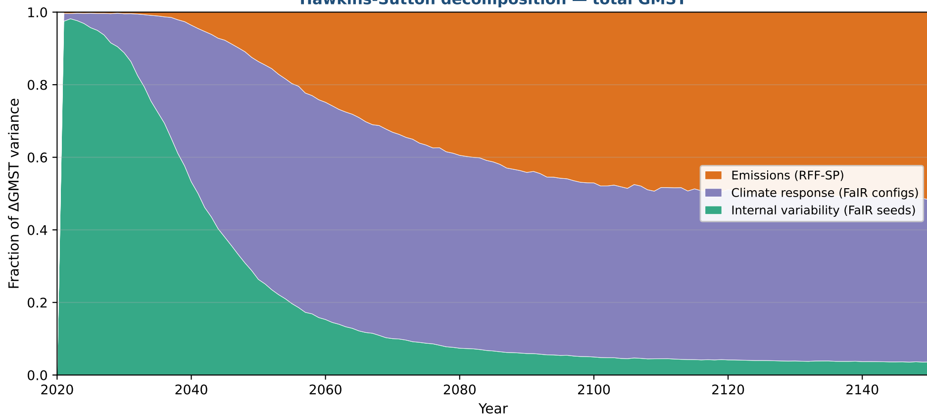
Hawkins-Sutton decomposition — total GMST
