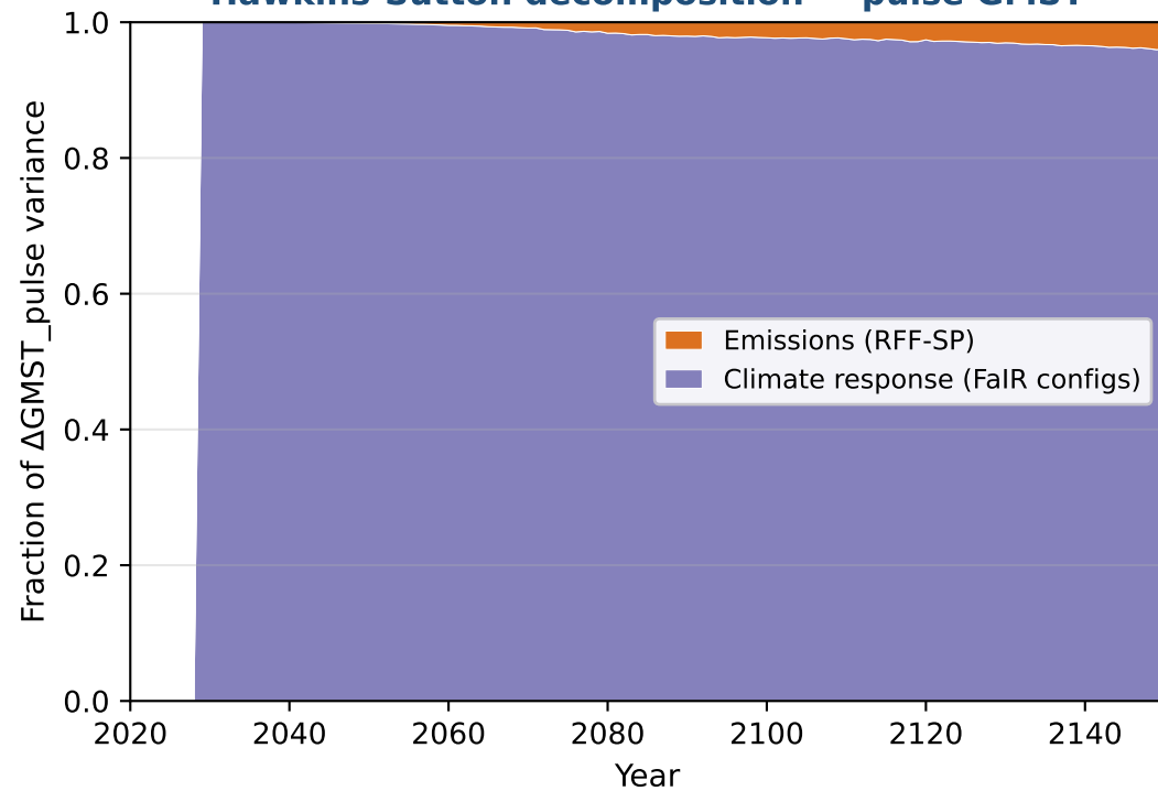
Hawkins-Sutton decomposition — pulse GMST
