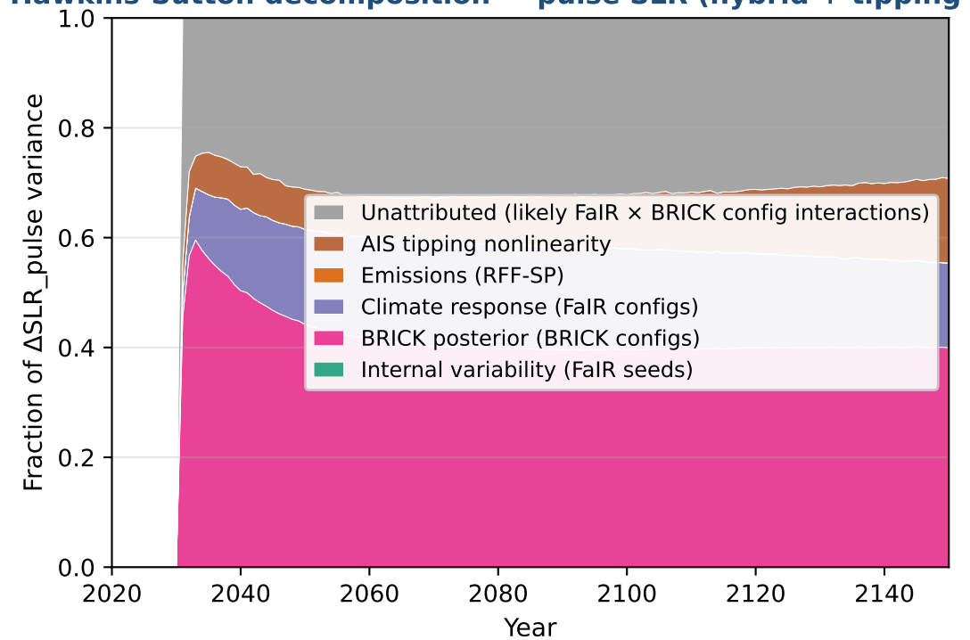
Hawkins-Sutton decomposition — pulse SLR (hybrid + tipping split)
