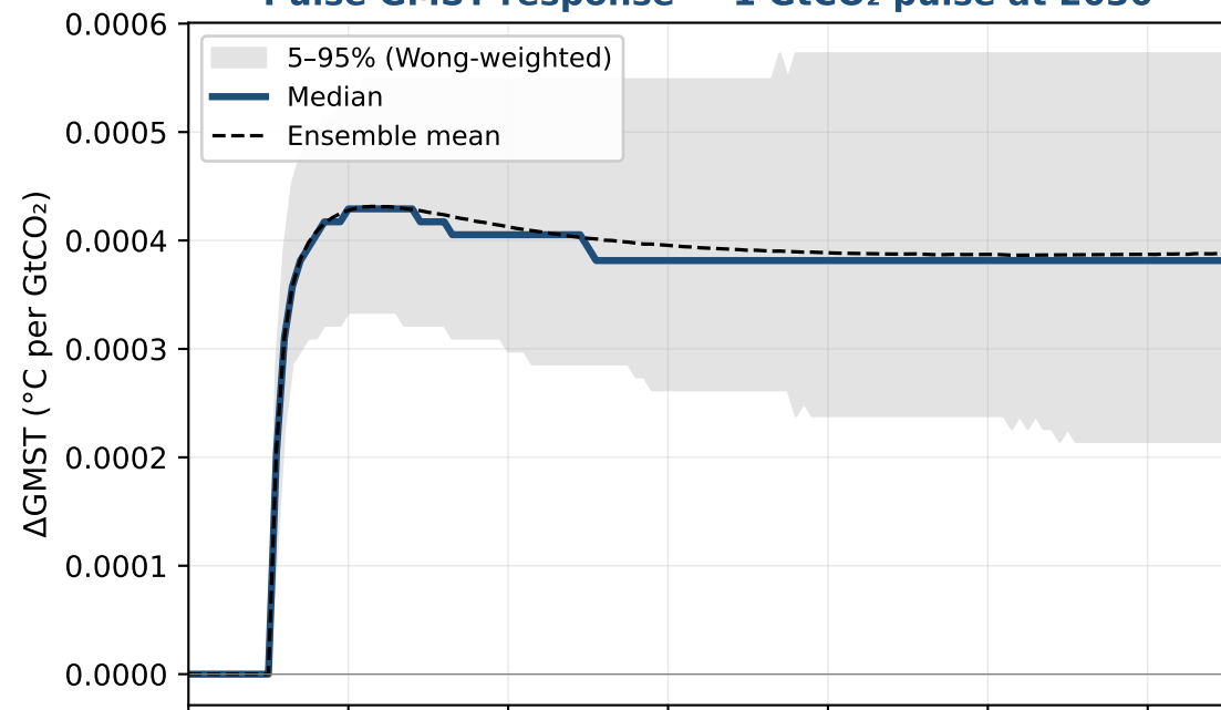
Pulse GMST response — 1 GtCO 2 pulse at 2030
