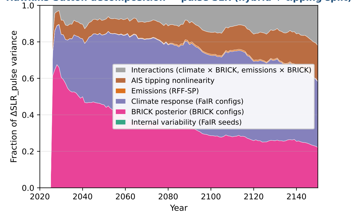
Hawkins-Sutton decomposition — pulse SLR (hybrid + tipping split)
