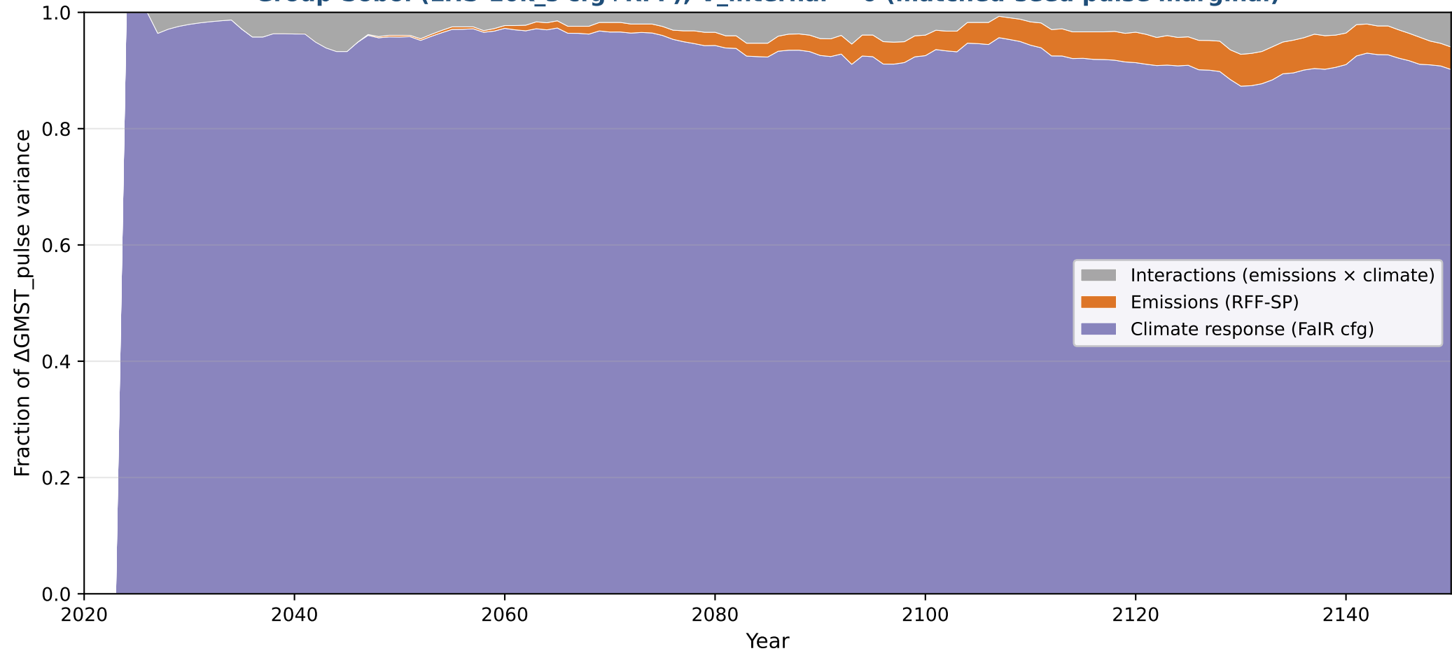
Pulse-marginal \Delta GMST (per GtCO 2 , 2030 pulse) Group-Sobol (LHS-10k_s cfg+RFF); V internal = 0 (matched-seed pulse marginal)
