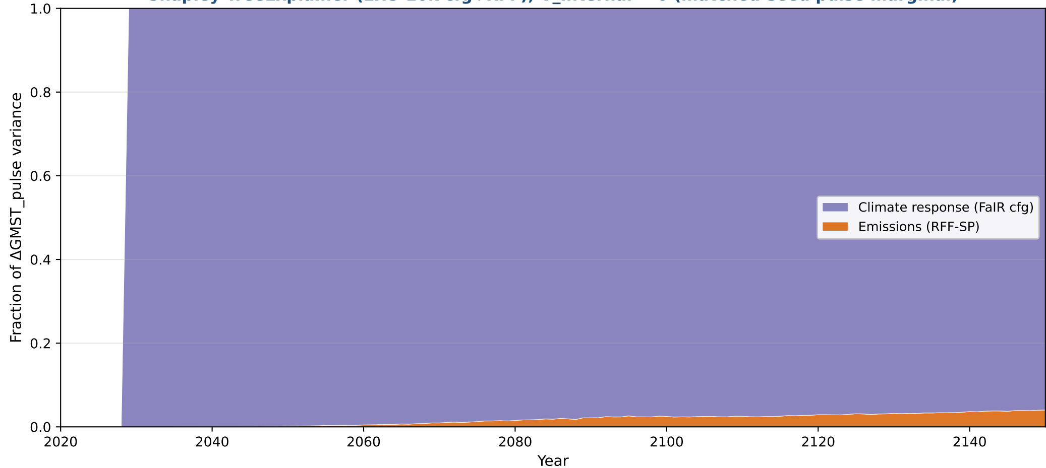
Pulse-marginal \Delta GMST (per GtCO 2 , 2030 pulse) Shapley TreeExplainer (LHS-10k cfg+RFF); V internal = 0 (matched-seed pulse marginal)
