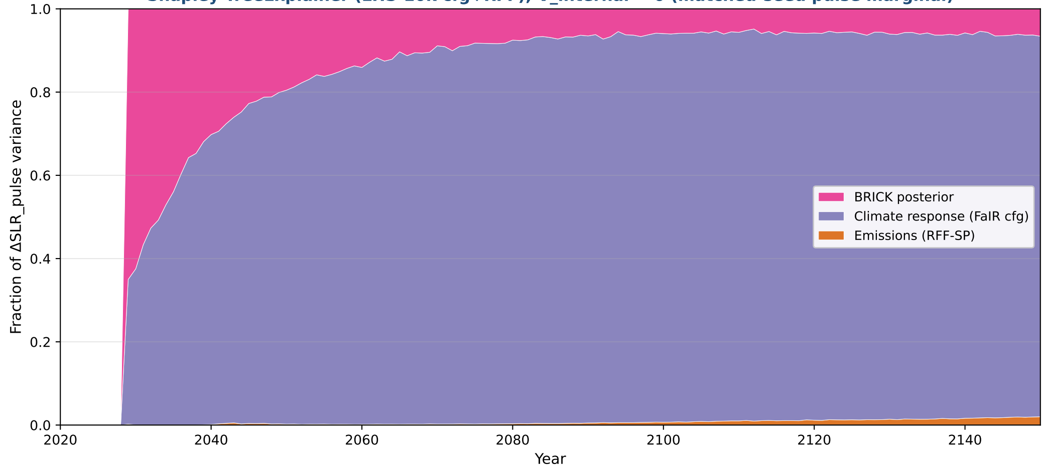
Pulse-marginal \Delta SLR (per GtCO 2 , 2030 pulse, linear regime) Shapley TreeExplainer (LHS-10k cfg+RFF); V internal = 0 (matched-seed pulse marginal)
