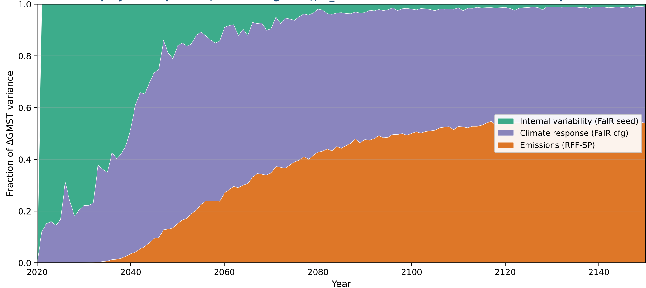
Total \Delta GMST (relative to 2020) Shapley TreeExplainer (LHS-10k cfg+RFF); V_internal from v1.4.5 ANOVA-18k seed replicates
