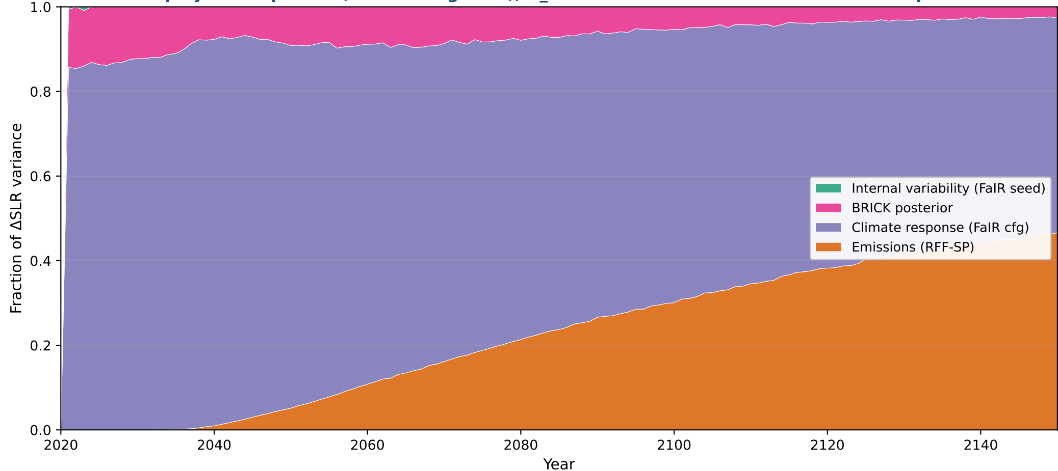
Total \Delta SLR (relative to 2020) Shapley TreeExplainer (LHS-10k cfg+RFF); V_internal from v1.4.5 ANOVA-18k seed replicates
