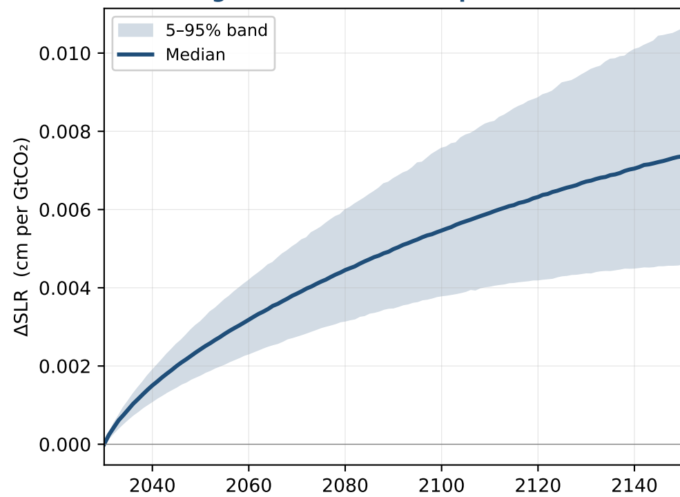
Marginal SLR — 1 GtCO 2 pulse at 2030
