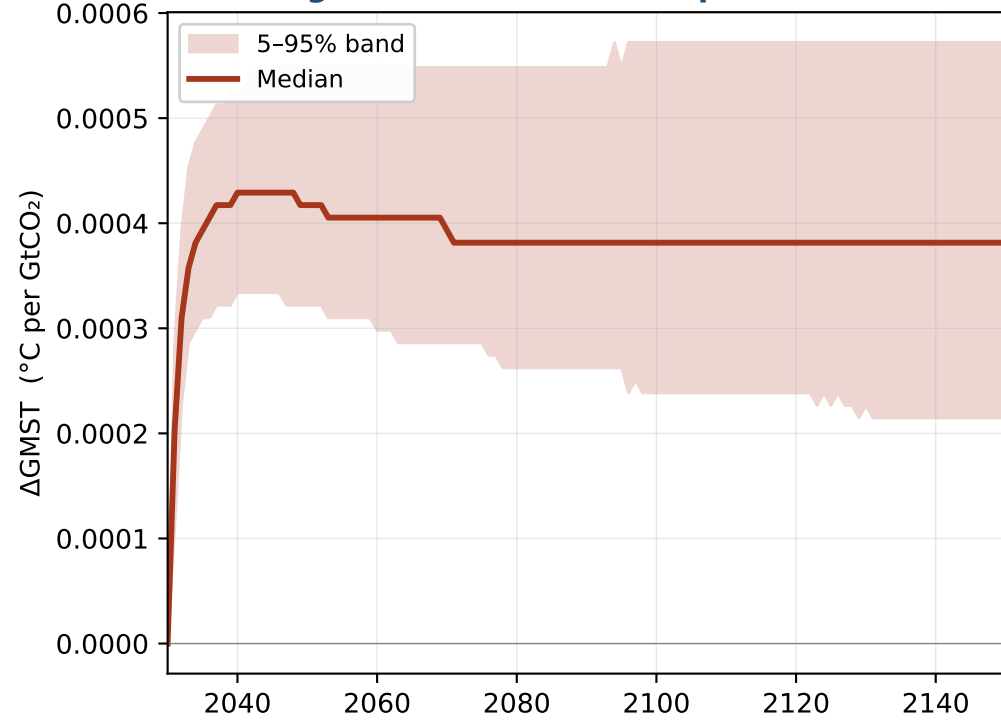
Marginal GMST — 1 GtCO 2 pulse at 2030
