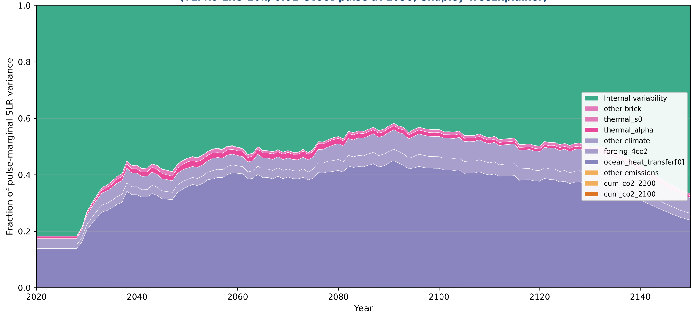
Pulse-marginal SLR variance — top-2 drivers per source axis (v1.4.5 LHS-10k, 0.01-GtCO 2 pulse at 2030; Shapley TreeExplainer)
