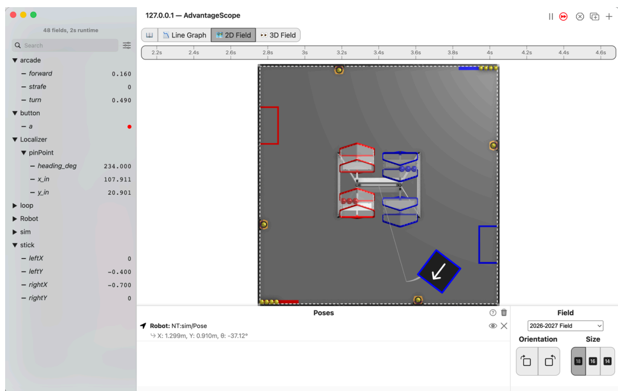
Figure 3.73. AdvantageScope's 2D Field with the robot right of where it started and turned partway round, with the list showing arcade/forward at 0.160, arcade/turn at 0.490, and pinPoint/x_in at 107.911, y_in at 20.901 and heading_deg at 234.
