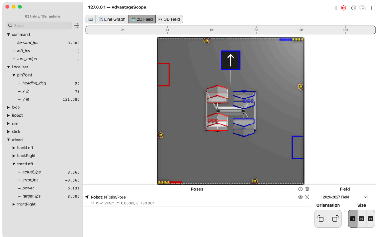
Figure 3.81. AdvantageScope's 2D Field with the robot near the top of the field, its arrow pointing up, and the list showing command/forward_ips at 8, pinPoint/y_in at 121.080, and wheel/frontLeft with target_ips at 8, actual_ips at 8.365, error_ips at -0.365 and power at 0.131.
