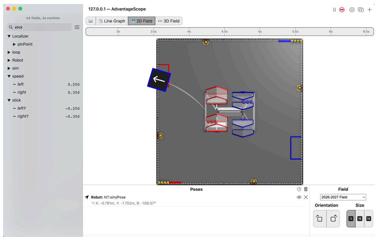
Figure 3.44. AdvantageScope's 2D Field connected to the simulator, with the robot NT:sim/Pose near the left wall after curving left from its start, speed/left reading 0.250 and speed/right 0.350.
