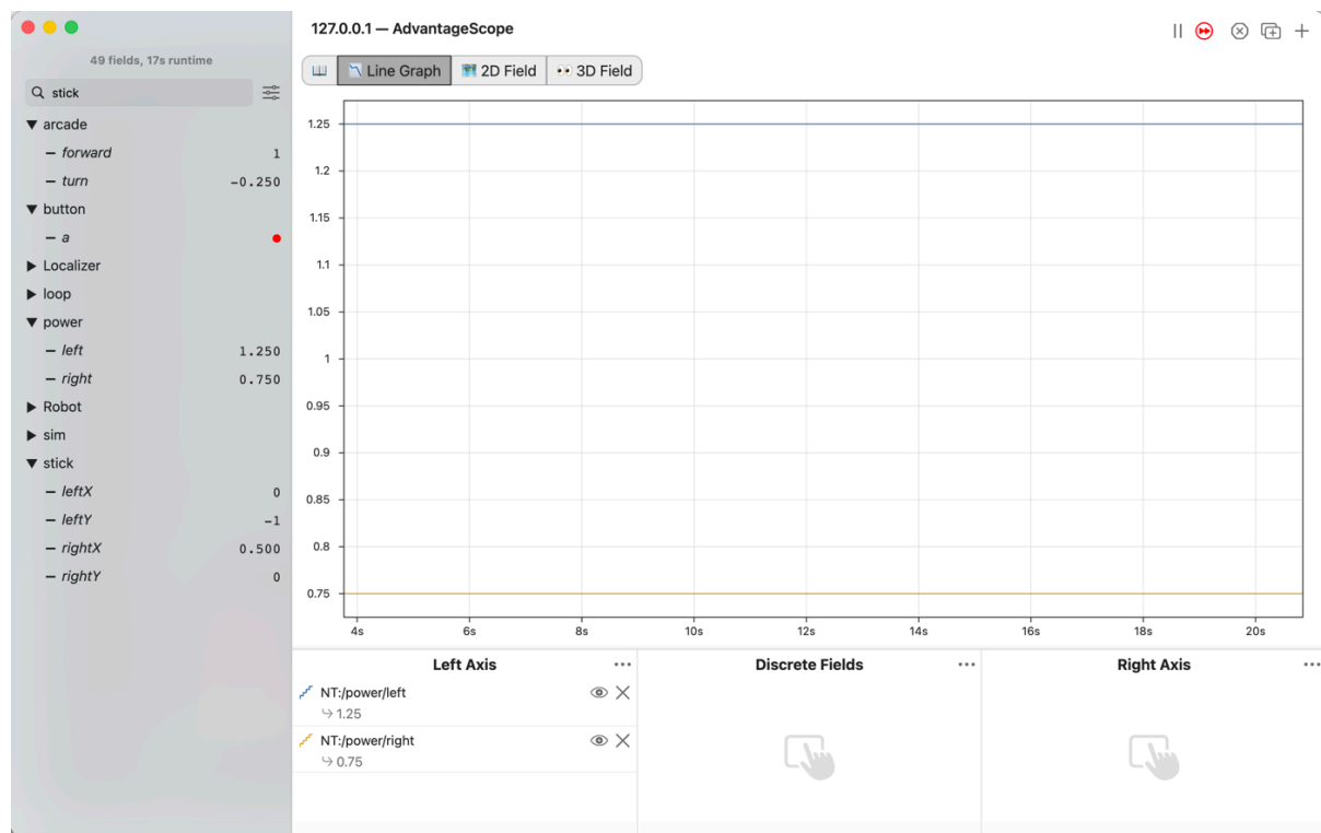
Figure 3.58. AdvantageScope’s Line Graph with NT:/power/left at 1.25 and NT:/power/right at 0.75 on Left Axis, and the list showing arcade/forward at 1 and arcade/turn at -0.250.
