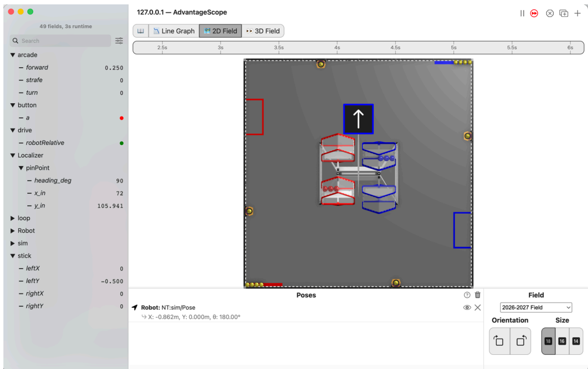
Figure 3.75. AdvantageScope's 2D Field with the robot above the middle of the field, its arrow pointing up the field, and the list showing drive/robotRelative green, arcade/forward at 0.250, and pinPoint / x_in at 72, y_in at 105.941 and heading_deg at 90.
