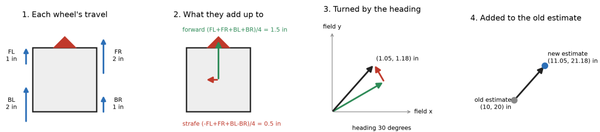
Figure 3.68. One loop of dead reckoning: the four wheel travels since the last loop, the forward and left arrows those add up to, the same pair turned to point along the robot's heading, and the old estimate with that pair added on the end.
