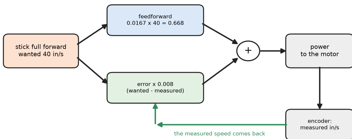
Figure 3.83. The loop drawn once round: the stick asking for 40 in/s, the feedforward guess at the power, the encoder's measured speed coming back, and the error being added in.
