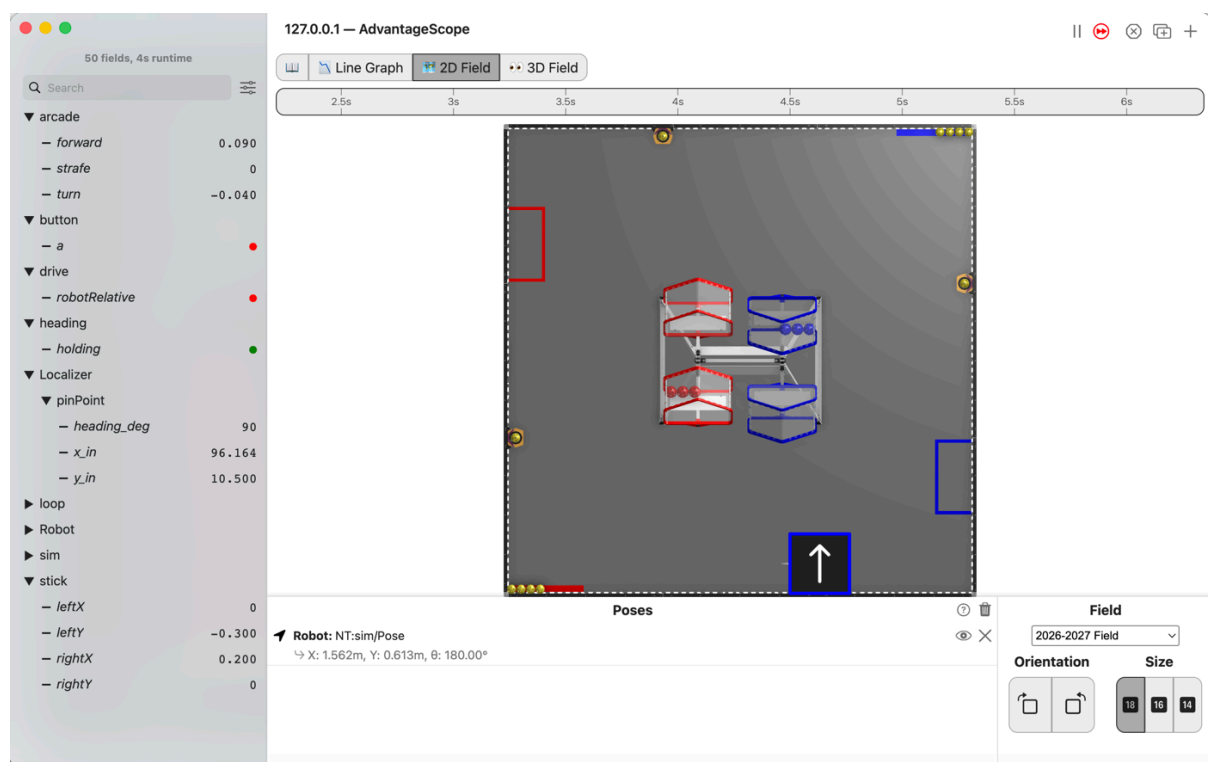
Figure 3.43. AdvantageScope's 2D Field with the robot near the bottom of the field, right of the middle, its arrow still pointing up the field, and the list showing arcade/turn at -0.040, heading/holding green, and pinPoint/heading_deg at 90 and x_in at 96.164.
