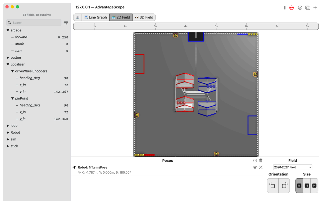
Figure 3.36. AdvantageScope's 2D Field with the robot at the top of the field, its arrow pointing up, and the list with the Localizer folder open: driveWheelEncoders and pinPoint both at x 72 and heading 90, and y_in at 142.367 and 142.360.
