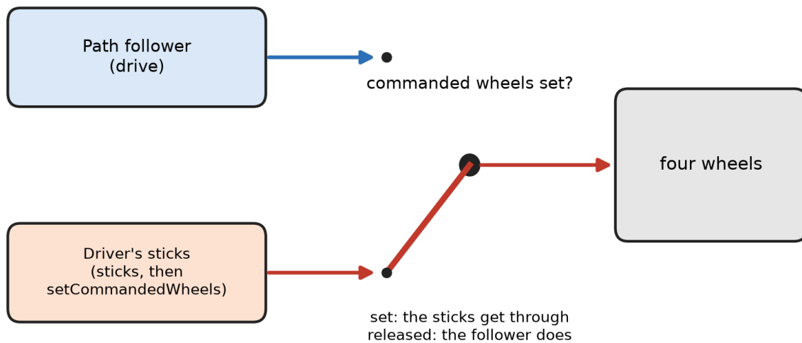
Figure 3.31. Two arrows reaching the same four wheels, one from the path follower and one from the driver's sticks, with the commanded-wheels switch between them showing which one gets through.
