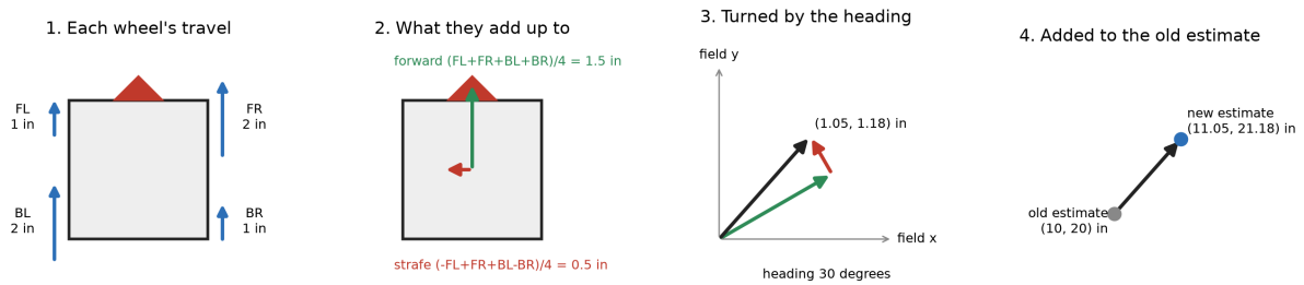
Figure 3.35. One loop of dead reckoning: the four wheel travels since the last loop, the forward and left arrows those add up to, the same pair turned to point along the robot's heading, and the old estimate with that pair added on the end.
