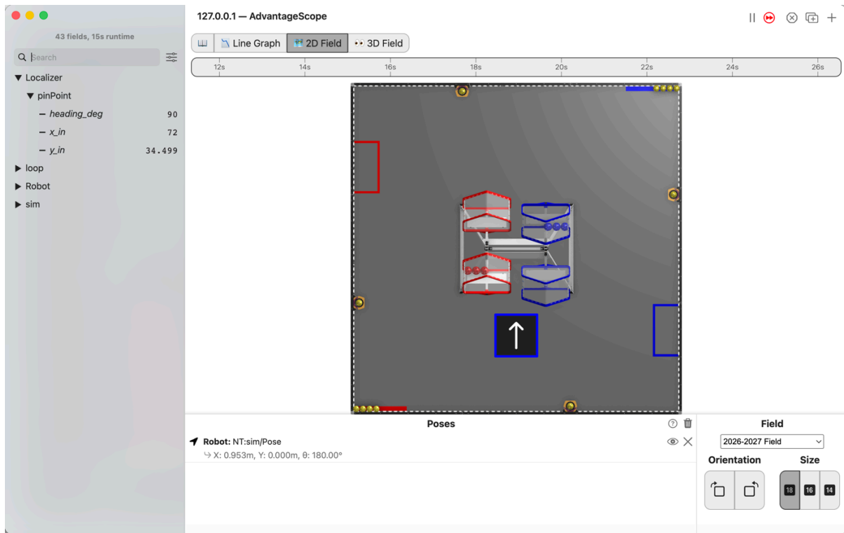
Figure 3.37. AdvantageScope's 2D Field with the robot stopped 24 inches up the field from where it started, its arrow pointing up the field, and the list showing pinPoint/y_in at 34.499, x_in at 72 and heading_deg at 90.
