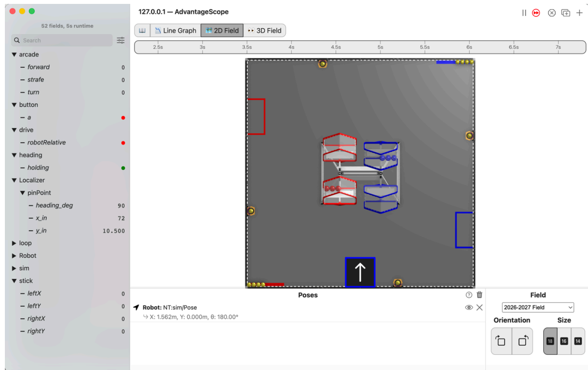
Figure 3.46. AdvantageScope's 2D Field with the robot at the bottom middle of the field, its arrow pointing up, and the list showing every stick at 0 and pinPoint/x_in at 72, y_in at 10.500 and heading_deg at 90.
