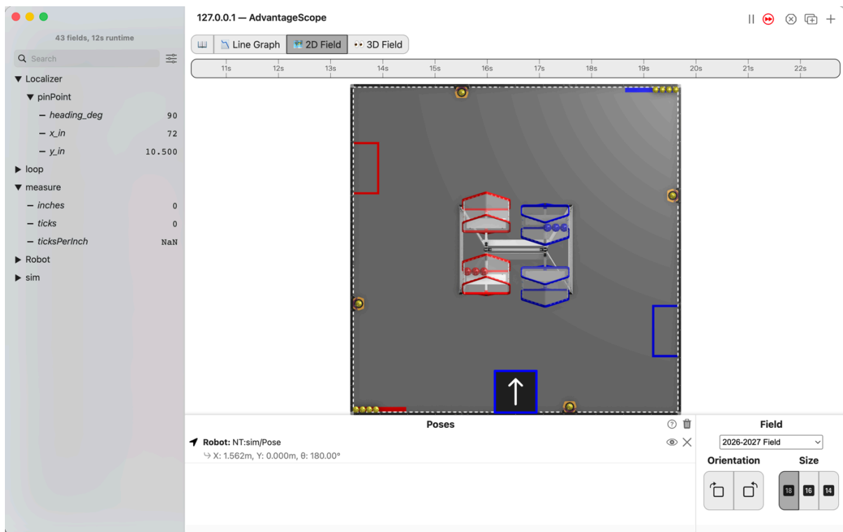
Figure 3.51. AdvantageScope’s 2D Field with the robot at the bottom middle of the field, its arrow pointing up, and the list showing pinPoint at x 72 , y 10.500 and heading 90 , and measure with inches and ticks at 0 and ticksPerInch at NaN .
