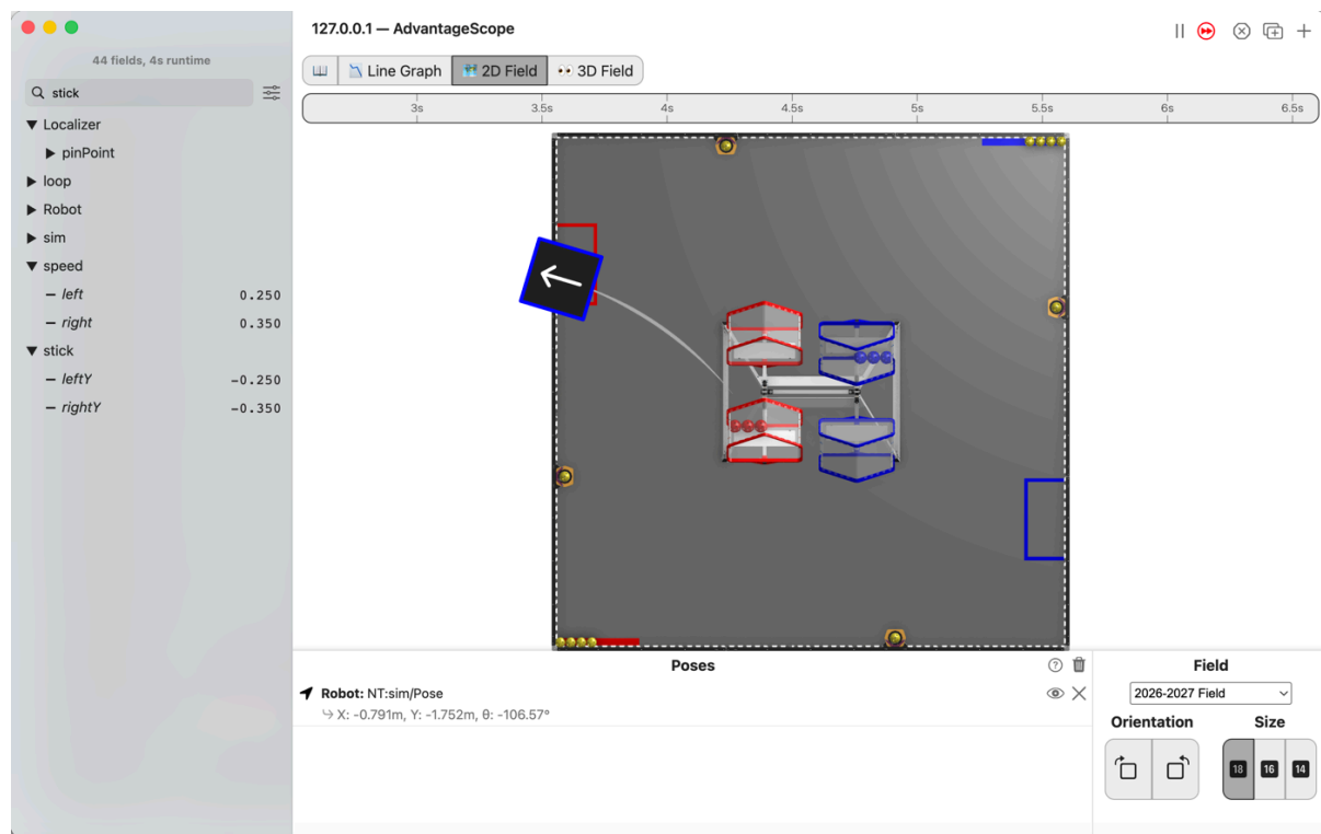
Figure 3.11. AdvantageScope's 2D Field connected to the simulator, with the robot NT:sim/Pose near the left wall after curving left from its start, speed/left reading 0.250 and speed/right 0.350.
