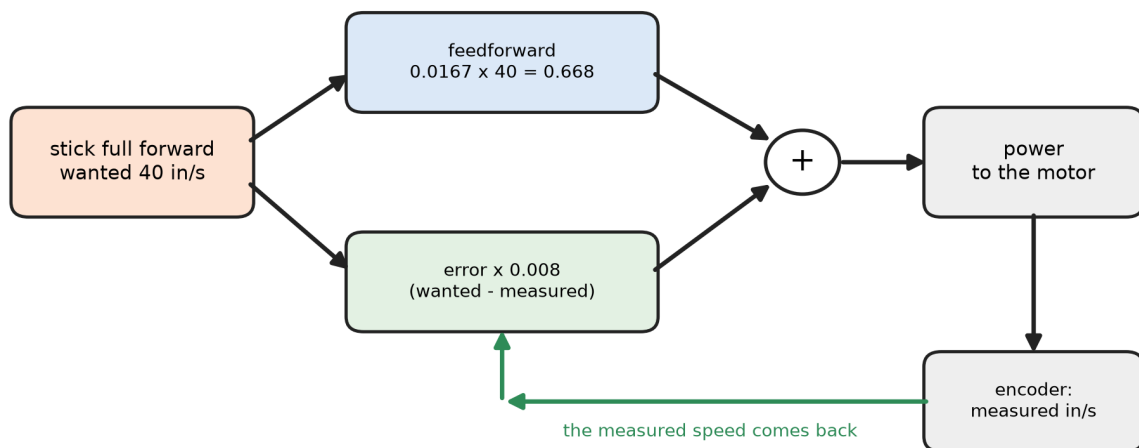
Figure 3.50. The loop drawn once round: the stick asking for 40 in/s, the feedforward guess at the power, the encoder's measured speed coming back, and the error being added in.
