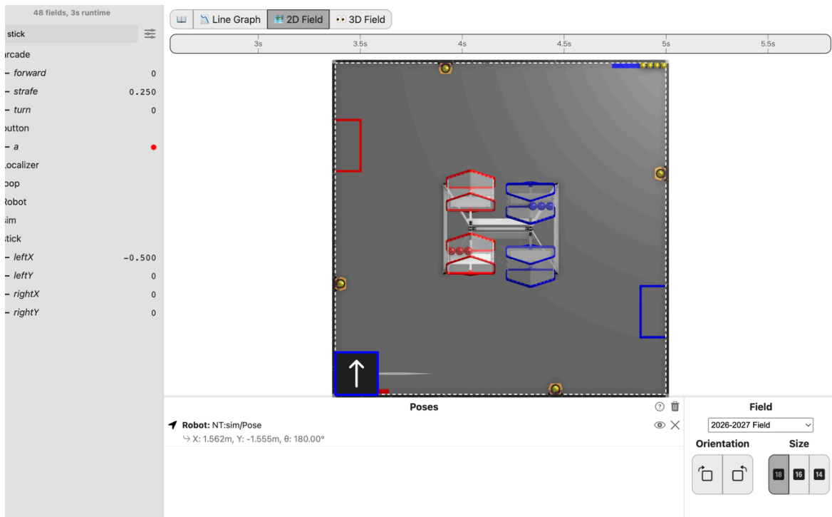
Figure 3.30. AdvantageScope's 2D Field with the robot NT:sim/Pose slid to its own left along the bottom edge, its nose still pointing the same way at 180.00^\circ , and the list showing arcade/strafe at 0.250, as in L090, with the path follower holding the drivetrain.
