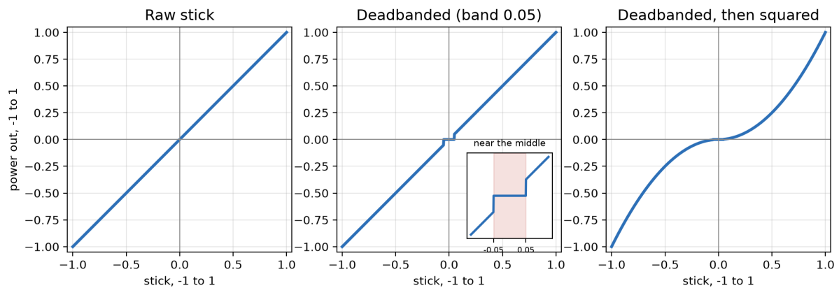
Figure 3.17. Three graphs side by side, each with the stick from -1 to 1 along the bottom and the power out from -1 to 1 up the side: the raw stick as a straight line, the deadbanded stick as a line with a flat step at the middle, and the squared stick as an S through the middle.
