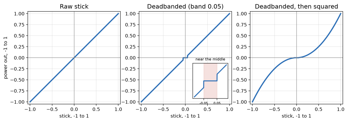
Figure 3.18. Three graphs side by side, each with the stick from -1 to 1 along the bottom and the power out from -1 to 1 up the side: the raw stick as a straight line, the deadbanded stick as a line with a flat step at the middle, and the squared stick as an S through the middle.
