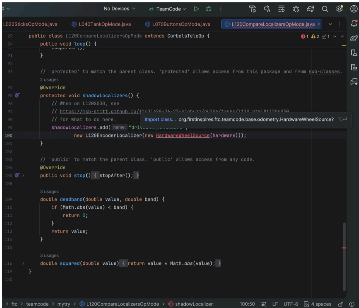
Figure 3.36. Android Studio with HardwareWheelSource underlined in red and the popup offering Import class... org.firstinspires.ftc.teamcode.base.odometry.HardwareWheelSource? with ⌘⇧I .
