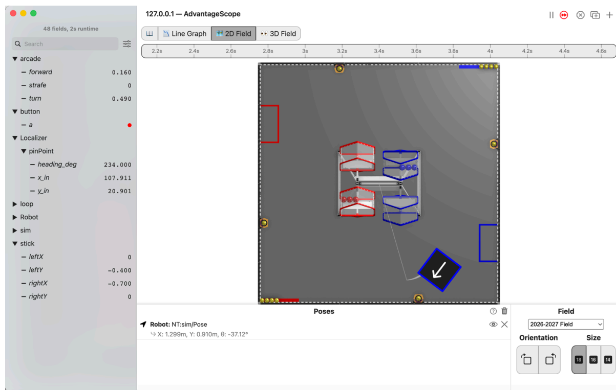
Figure 3.42. AdvantageScope's 2D Field with the robot right of where it started and turned partway round, with the list showing arcade/forward at 0.160, arcade/turn at 0.490, and pinPoint/x_in at 107.911, y_in at 20.901 and heading_deg at 234.
