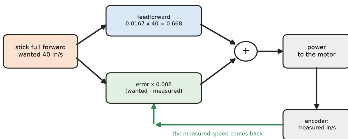
Figure 3.50. The loop drawn once round: the stick asking for 40 in/s, the feedforward guess at the power, the encoder's measured speed coming back, and the error being added in.
