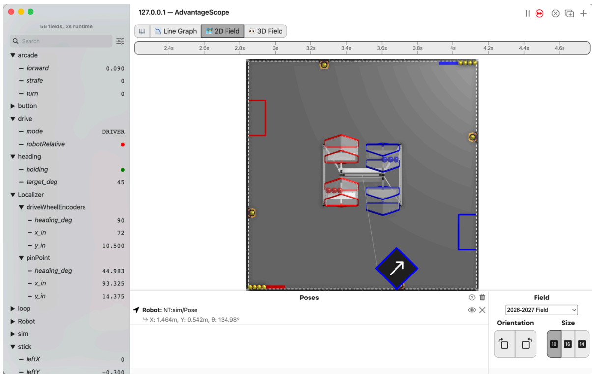
Figure 2.46. AdvantageScope's 2D Field with the robot near the bottom of the field, right of the middle, its arrow pointing up and to the right, and the list showing drive/mode at DRIVER, heading/holding green and target_deg at 45, driveWheelEncoders at x 72, y 10.500 and heading 90, and pinPoint at x 93.325, y 14.375 and heading 44.983.
