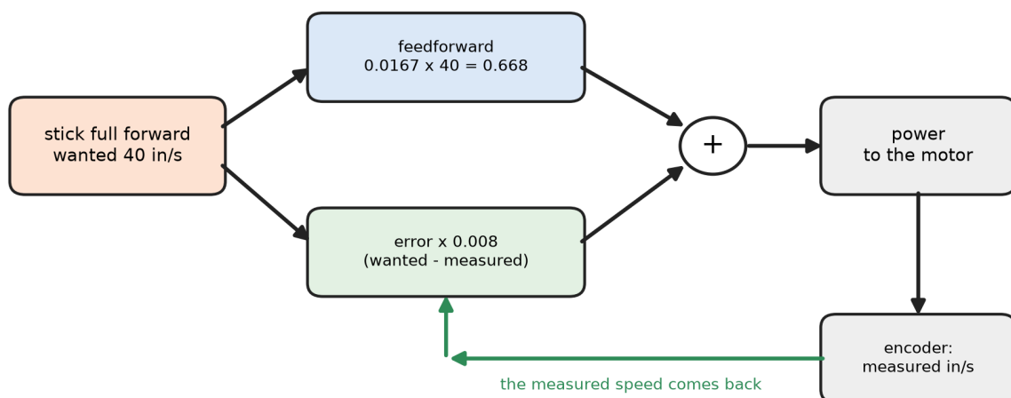
Figure 2.49. The loop drawn once round: the stick asking for 40 in/s, the feedforward guess at the power, the encoder's measured speed coming back, and the error being added in.
