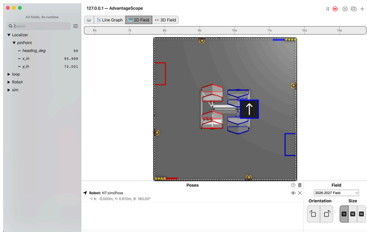
Figure 2.38. AdvantageScope's 2D Field with the robot stopped right of the middle of the field, its arrow still pointing up the field, and the list showing pinPoint/x_in at 95.999, y_in at 72.001 and heading_deg at 90.
