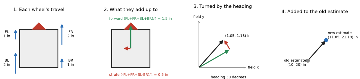
Figure 2.38. One loop of dead reckoning: the four wheel travels since the last loop, the forward and left arrows those add up to, the same pair turned to point along the robot’s heading, and the old estimate with that pair added on the end.
