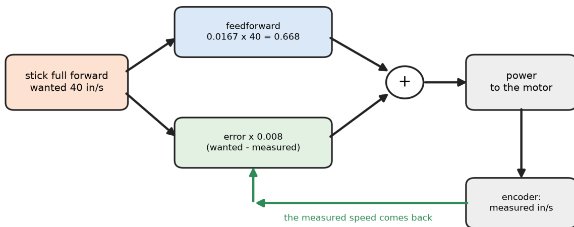
Figure 2.52. The loop drawn once round: the stick asking for 40 in/s, the feedforward guess at the power, the encoder's measured speed coming back, and the error being added in.
