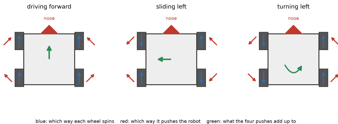
Figure 2.30. The robot from above, three times: driving forward, sliding left and turning left. On each wheel, an arrow for the way it spins and an arrow at 45 degrees for the way it pushes the robot, and in the middle one arrow for where the four pushes add up to.
