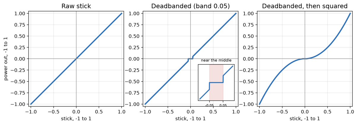
Figure 2.18. Three graphs side by side, each with the stick from -1 to 1 along the bottom and the power out from -1 to 1 up the side: the raw stick as a straight line, the deadbanded stick as a line with a flat step at the middle, and the squared stick as an S through the middle.
