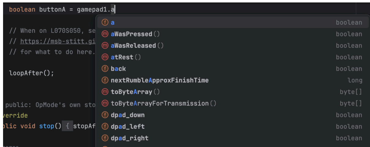
Figure 2.22. The list under gamepad1.a , offering a marked boolean first, then aWasPressed() and aWasReleased() .
