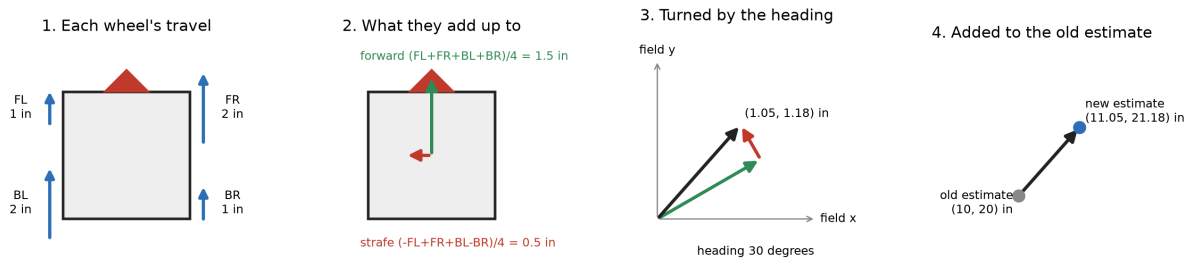
Figure 3.35. One loop of dead reckoning: the four wheel travels since the last loop, the forward and left arrows those add up to, the same pair turned to point along the robot's heading, and the old estimate with that pair added on the end.
