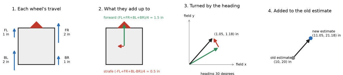
Figure 3.37. One loop of dead reckoning: the four wheel travels since the last loop, the forward and left arrows those add up to, the same pair turned to point along the robot’s heading, and the old estimate with that pair added on the end.
