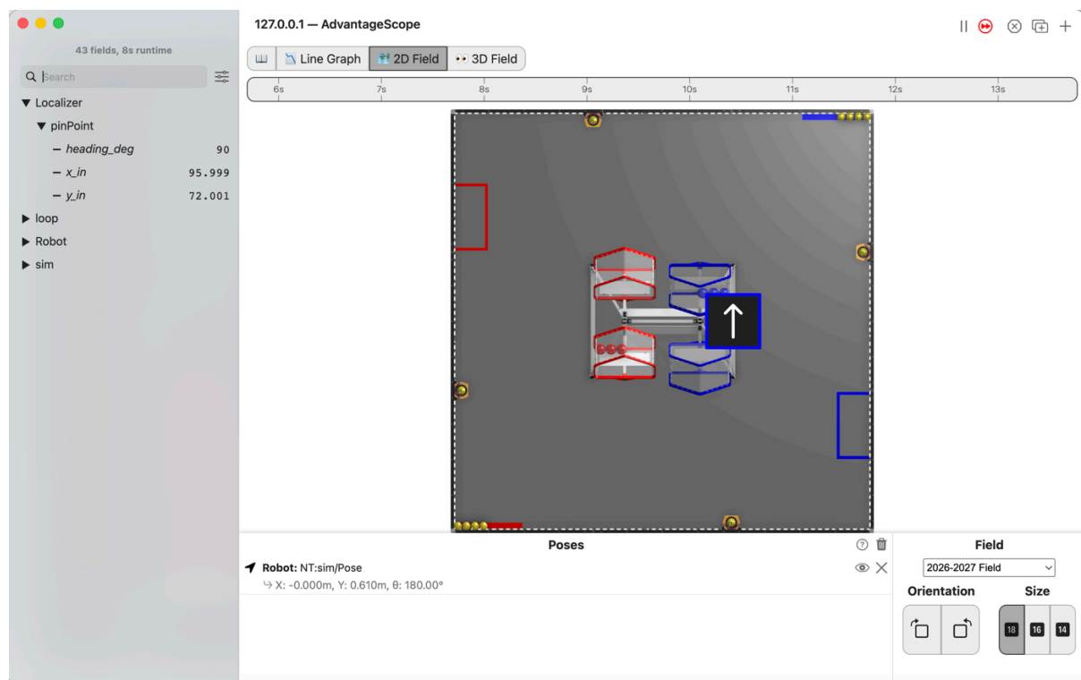
Figure 3.41. AdvantageScope's 2D Field with the robot stopped right of the middle of the field, its arrow still pointing up the field, and the list showing pinPoint/x_in at 95.999, y_in at 72.001 and heading_deg at 90.
