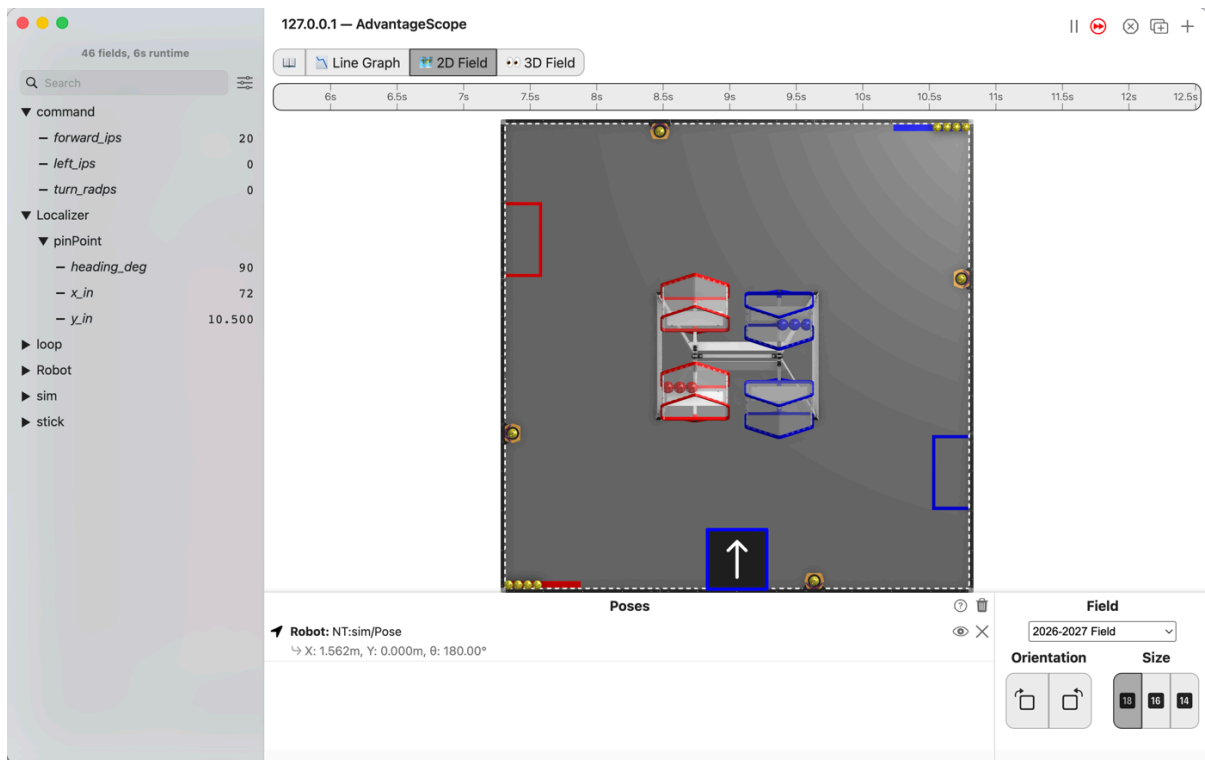
Figure 3.51. AdvantageScope's 2D Field with the robot at the bottom middle of the field, its arrow pointing up, and the list showing command/forward_ips at 20, left_ips and turn_radps at 0, and pinPoint at x 72, y 10.500 and heading 90, with no wheel folder.
