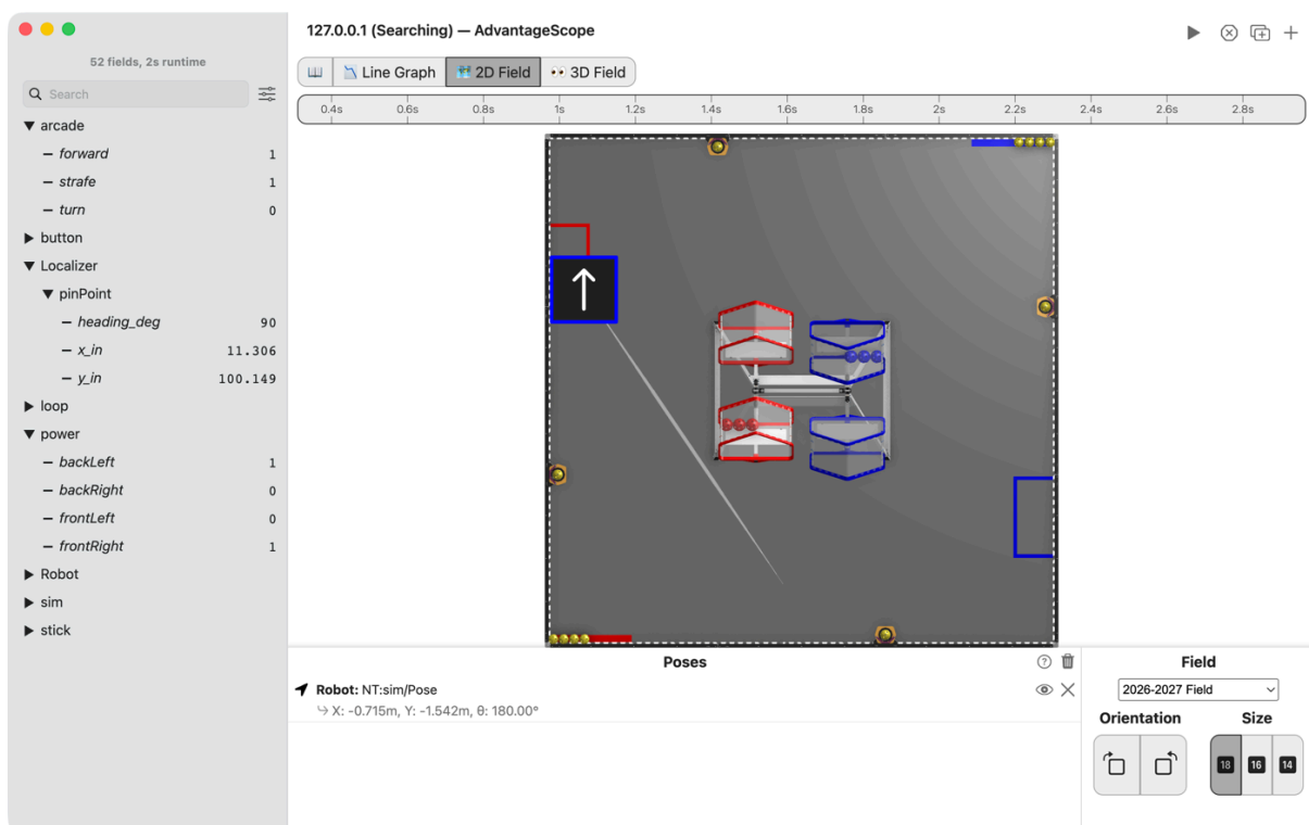
Figure 3.29. AdvantageScope's 2D Field and list with the left stick in the forward-left corner: arcade/forward and arcade/strafe at 1, power/frontRight and power/backLeft at 1, power/frontLeft and power/backRight at 0, and the robot's heading still 180.00°.
