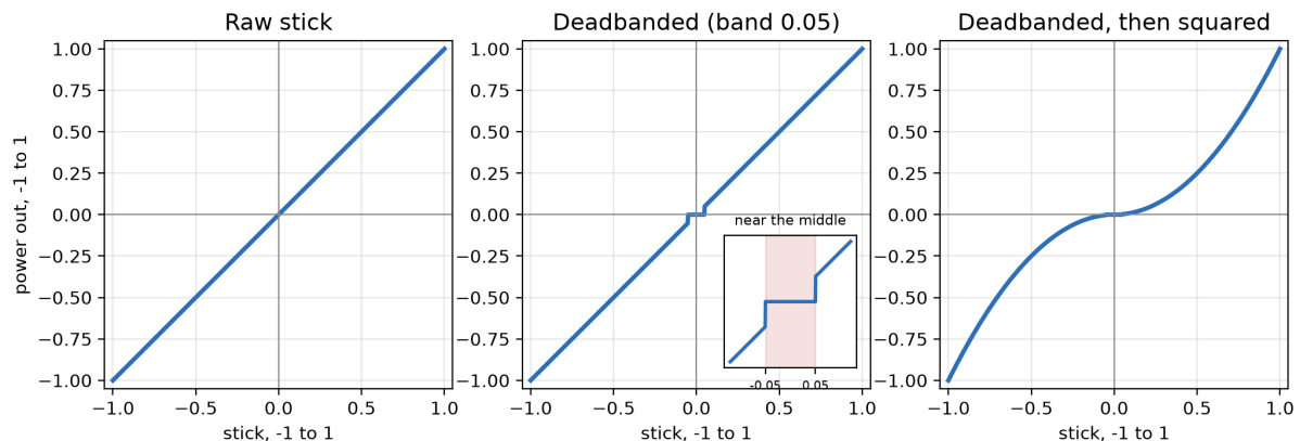
Figure 3.18. Three graphs side by side, each with the stick from -1 to 1 along the bottom and the power out from -1 to 1 up the side: the raw stick as a straight line, the deadbanded stick as a line with a flat step at the middle, and the squared stick as an S through the middle.
