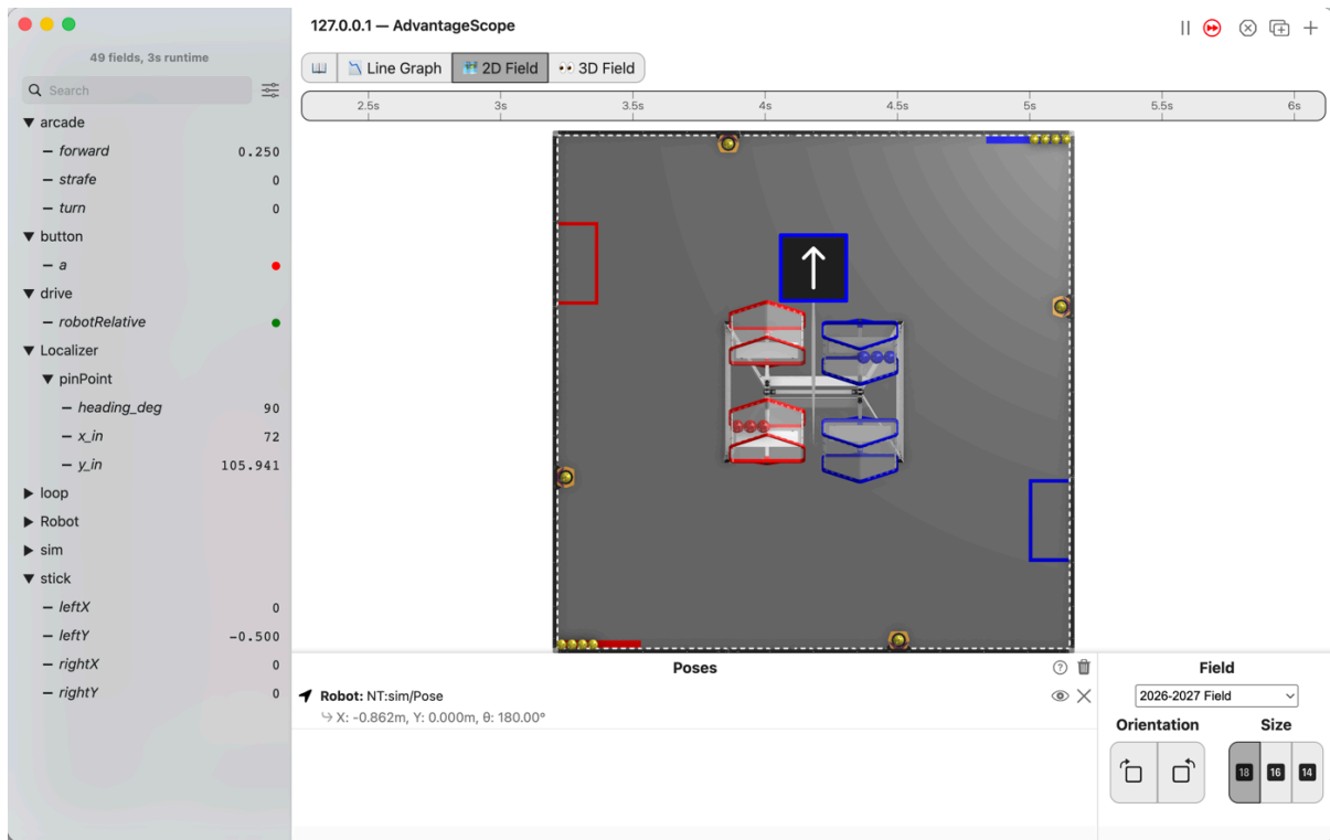
Figure 3.44. AdvantageScope's 2D Field with the robot above the middle of the field, its arrow pointing up the field, and the list showing drive/robotRelative green, arcade/forward at 0.250, and pinPoint /x_in at 72, y_in at 105.941 and heading_deg at 90.
