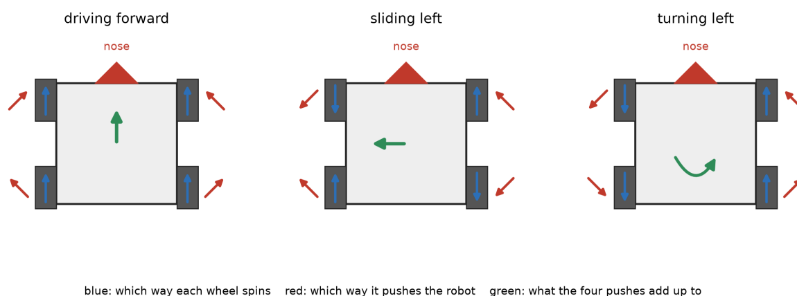
Figure 3.30. The robot from above, three times: driving forward, sliding left and turning left. On each wheel, an arrow for the way it spins and an arrow at 45 degrees for the way it pushes the robot, and in the middle one arrow for where the four pushes add up to.
