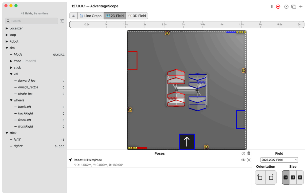
Figure 3.8. AdvantageScope's 2D Field with the robot NT:sim/Pose at its start. The list shows the four sim/wheels at 0, stick/leftY at -1 and stick/rightY at 0.5.
