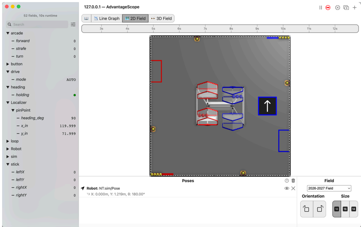
Figure 3.47. AdvantageScope's 2D Field with the robot right of the middle of the field, its arrow pointing up the field, and the list showing drive/mode at AUTO, every stick at 0, and pinPoint/x_in at 119.999, y_in at 71.999 and heading_deg at 90.
