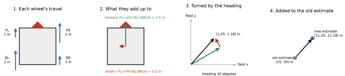
Figure 2.35. One loop of dead reckoning: the four wheel travels since the last loop, the forward and left arrows those add up to, the same pair turned to point along the robot’s heading, and the old estimate with that pair added on the end.
