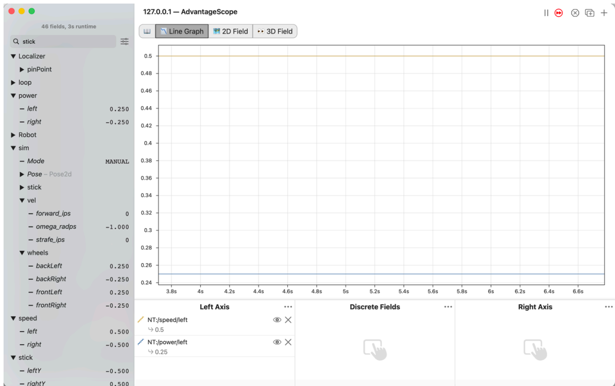
Figure 2.19. AdvantageScope's Line Graph with NT:/speed/left at 0.5 and NT:/power/left at 0.25, and the list showing power/right at -0.250 beside speed/right at -0.500.
