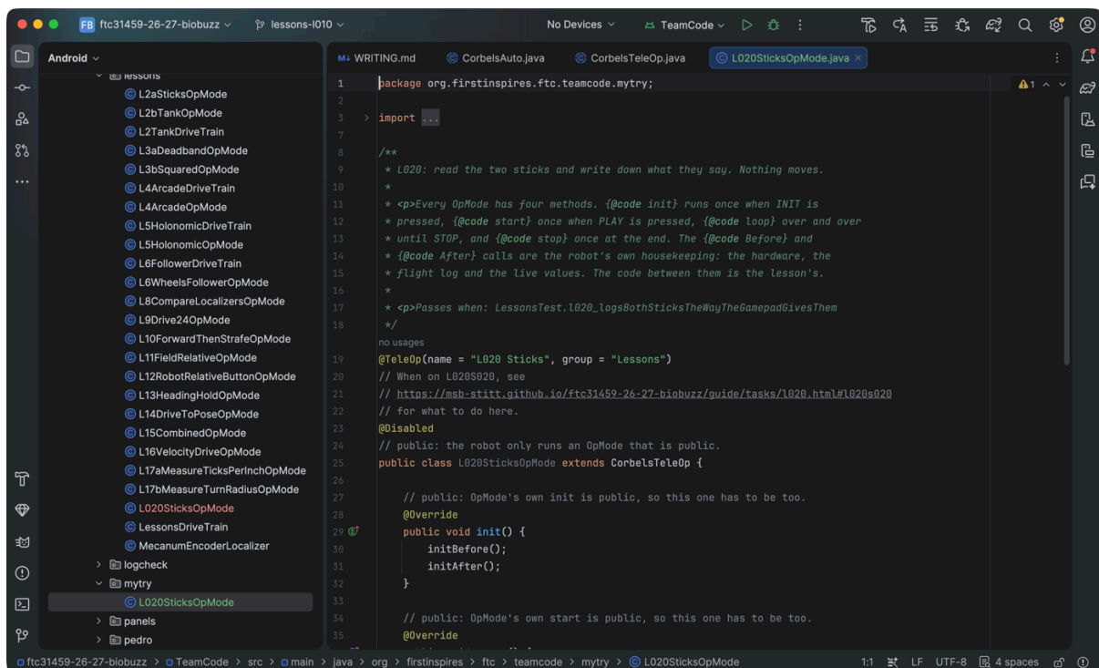
Figure 2.3. The Project window with lessons and the new mytry folder both open, L020SticksOpMode in each, and the copy open in the editor with its first line ending in mytry; .
