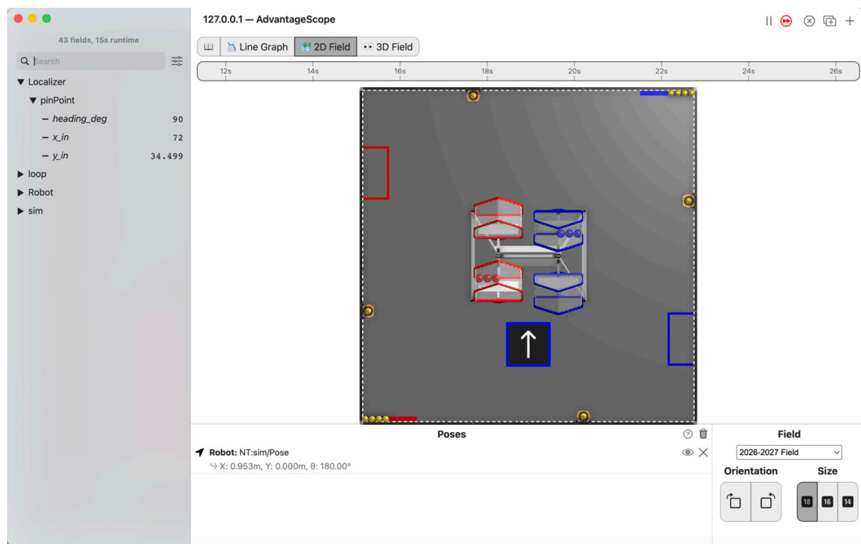
Figure 2.37. AdvantageScope's 2D Field with the robot stopped 24 inches out from the back wall, its arrow pointing up the field, and the list showing pinPoint/y_in at 34.499, x_in at 72 and heading_deg at 90.
