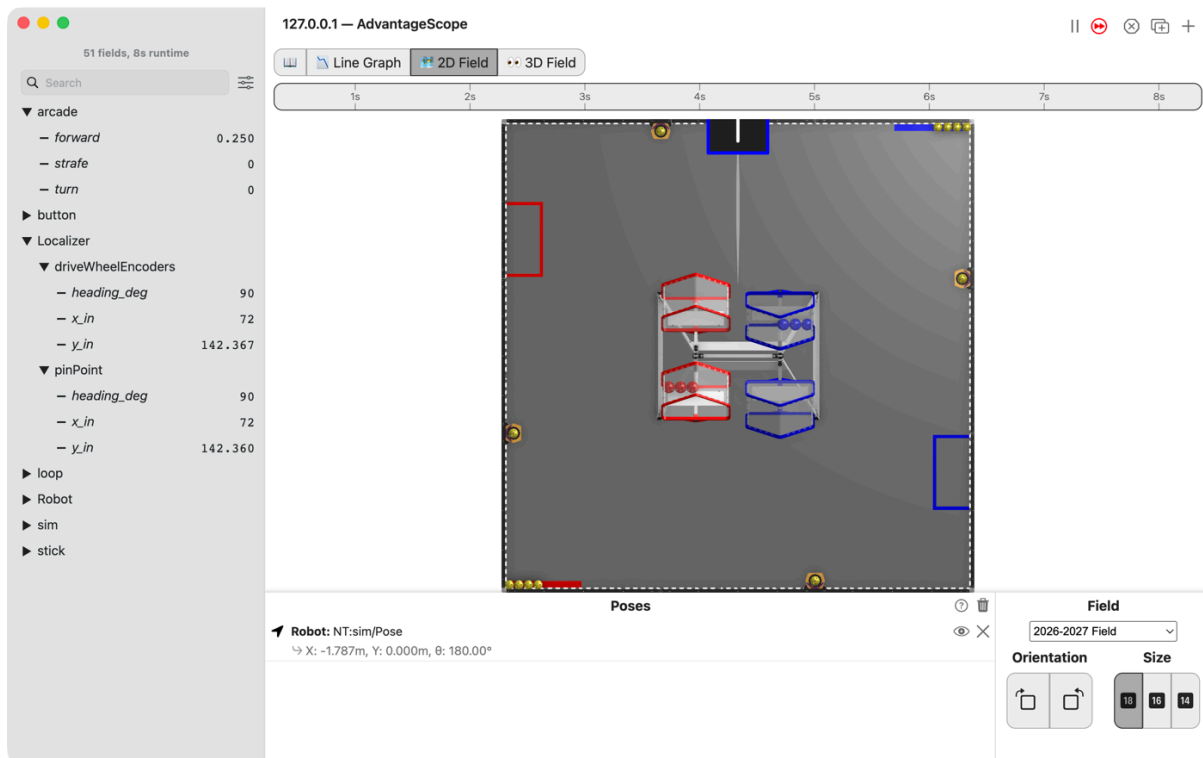
Figure 2.36. AdvantageScope's 2D Field with the robot at the top of the field, its arrow pointing up, and the list with the Localizer folder open: driveWheelEncoders and pinPoint both at x 72 and heading 90, and y\_in at 142.367 and 142.360.
