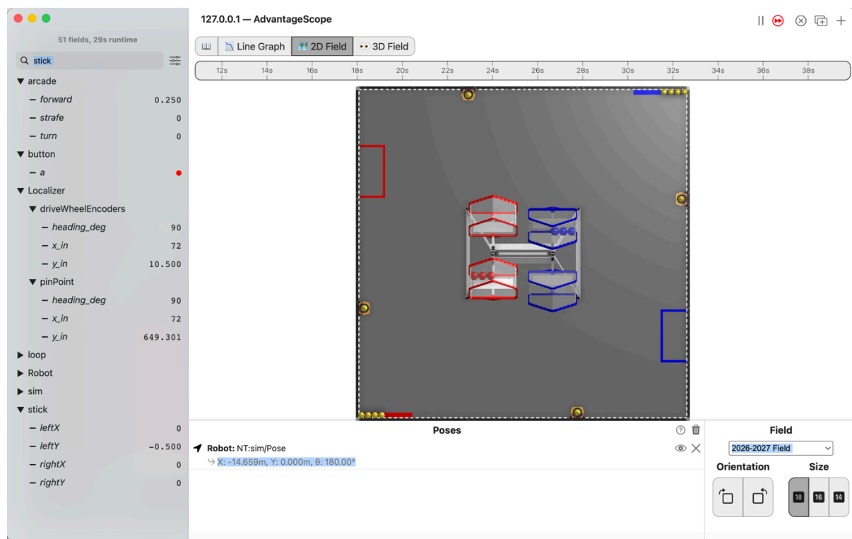
Figure 2.33. AdvantageScope's list with the Localizer folder open: pinPoint/y_in climbing past 600 while the robot drives forward, and driveWheelEncoders still at x 72, y 10.5 and heading 90, where it started.
