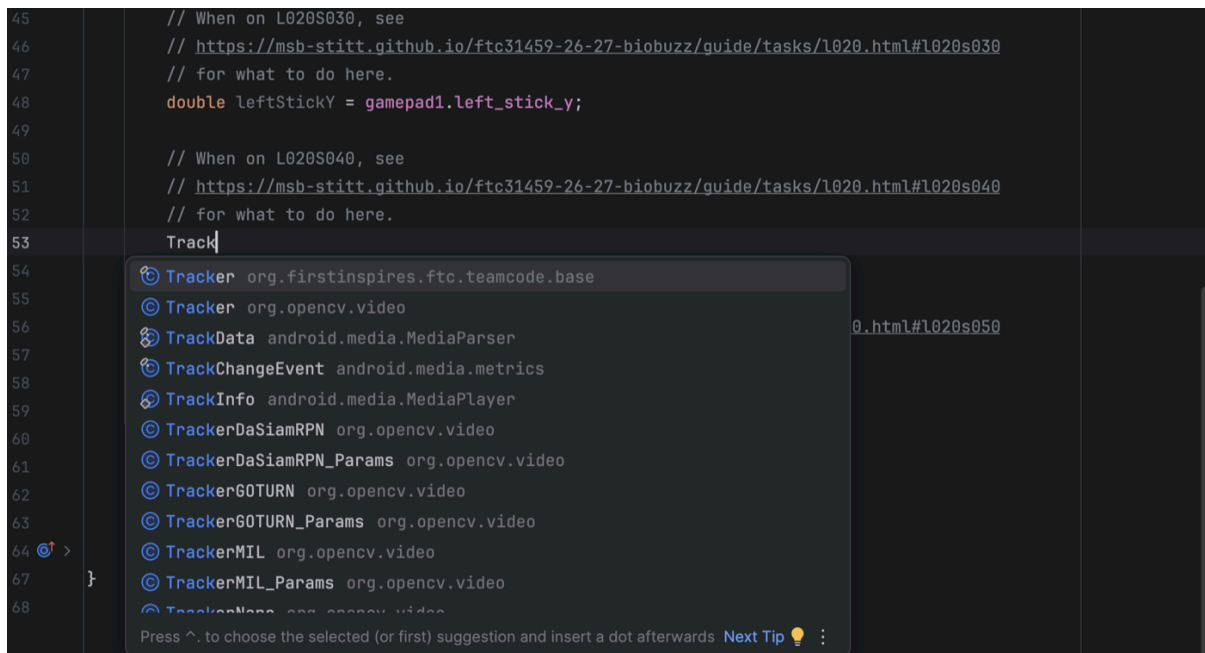
Figure 2.7. The list under Tracker , with Tracker from org.firstinspires.ftc.teamcode.base highlighted at the top and Tracker from org.opencv.video under it.
