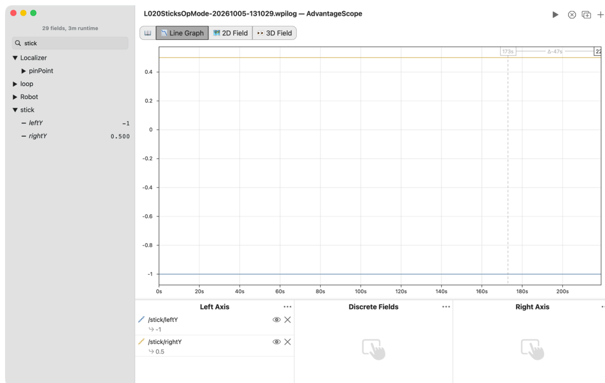
Figure 2.8. AdvantageScope's Line Graph of the flight log L020SticksOpMode-...wpilog , with /stick/leftY at -1 and /stick/rightY at 0.5 for the whole run.
