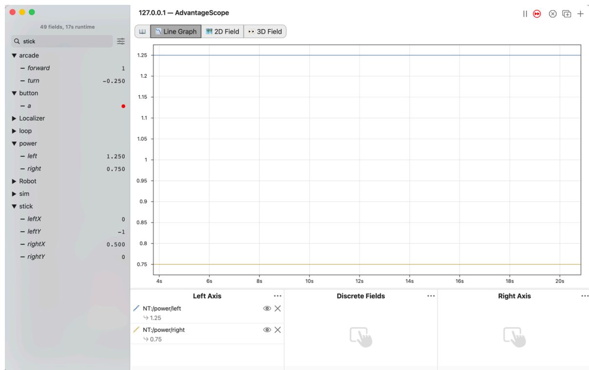
Figure 2.25. AdvantageScope's Line Graph with NT:/power/left at 1.25 and NT:/power/right at 0.75 on Left Axis , and the list showing arcade/forward at 1 and arcade/turn at -0.250.
