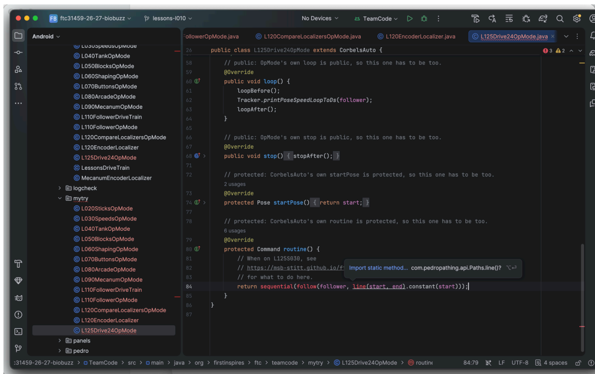
Figure 2.38. Android Studio with sequential , follow and line underlined in red and the popup offering Import static method... com.pedropathapi.Paths.line()? with ⌘↵ .
