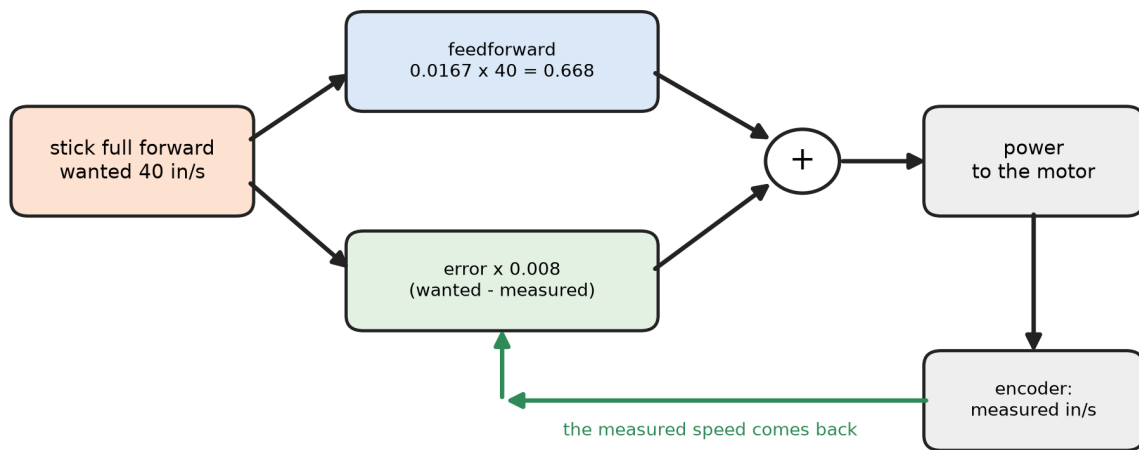
Figure 2.53. The loop drawn once round: the stick asking for 40 in/s, the feedforward guess at the power, the encoder's measured speed coming back, and the error being added in.
