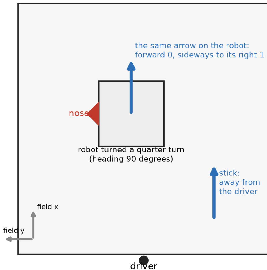
Figure 2.44. The field from above with the driver at the bottom, the robot turned a quarter turn, the stick's direction as an arrow on the field, and the same arrow drawn again on the robot showing what forward and sideways it turns into.
