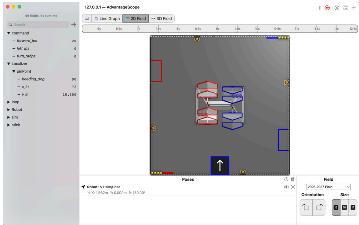
Figure 2.52. AdvantageScope's 2D Field with the robot at the bottom middle of the field, its arrow pointing up, and the list showing command/forward_ips at 20, left_ips and turn_radps at 0, and pinPoint at x 72, y 10.500 and heading 90, with no wheel folder.
