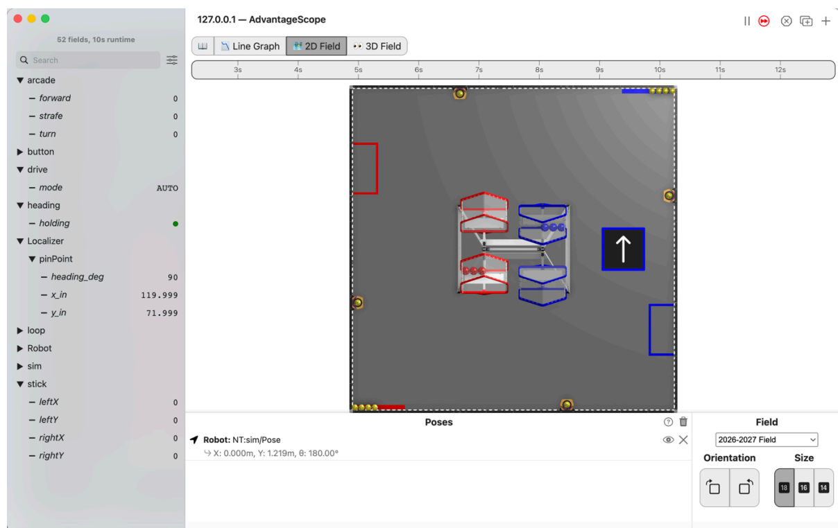
Figure 2.48. AdvantageScope's 2D Field with the robot right of the middle of the field, its arrow pointing up the field, and the list showing drive/mode at AUTO, every stick at 0, and pinPoint/x_in at 119.999, y_in at 71.999 and heading_deg at 90.
