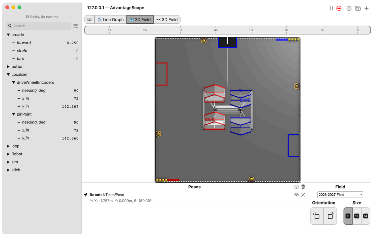
Figure 2.39. AdvantageScope's 2D Field with the robot at the top of the field, its arrow pointing up, and the list with the Localizer folder open: driveWheelEncoders and pinPoint both at x 72 and heading 90, and y_in at 142.367 and 142.360.
