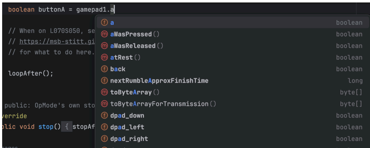
Figure 3.21. The list under gamepad1.a , offering a marked boolean first, then aWasPressed() and aWasReleased() .
