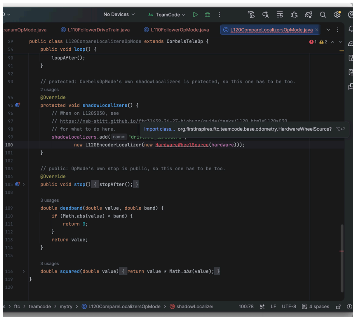
Figure 3.34. Android Studio with HardwareWheelSource underlined in red and the popup offering Import
