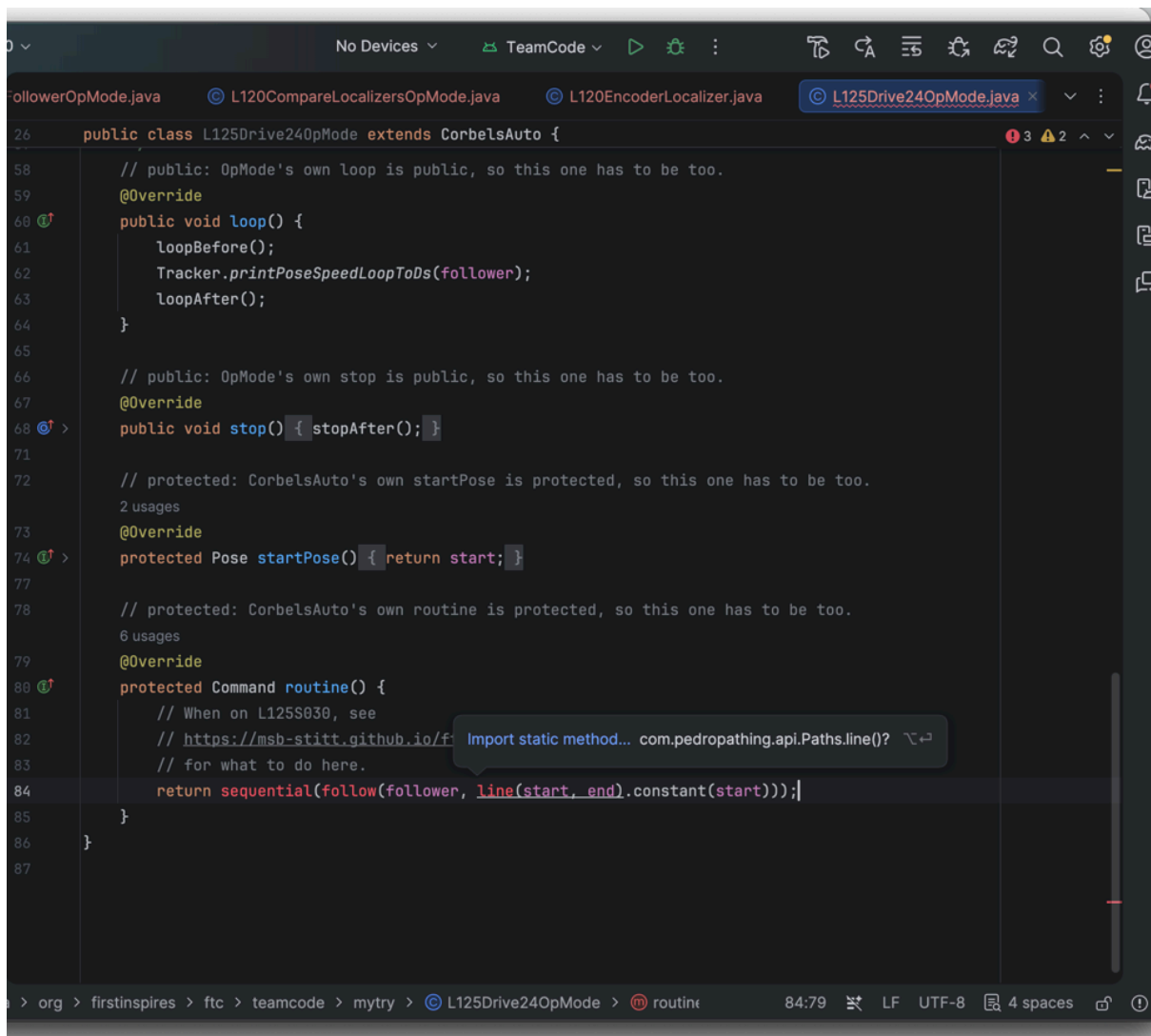
Figure 3.38. Android Studio with sequential, follow and line underlined in red and the popup offering Import static method... com.pedropathapi.Paths.line() ? with \u2197\u2190 .
