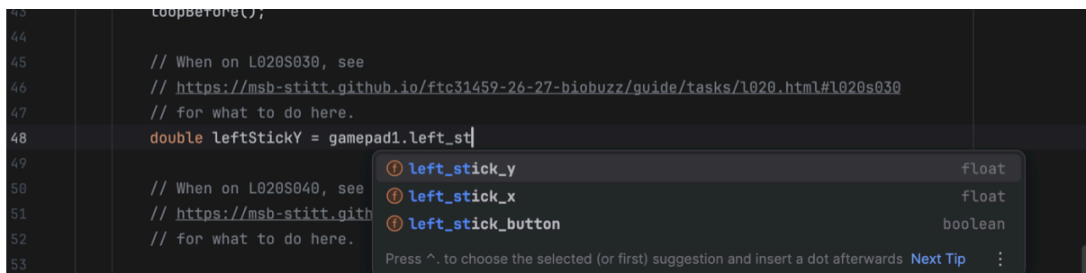
Figure 3.4. The list under gamepad1. after typing left_st , with left_stick_y highlighted and marked float.
