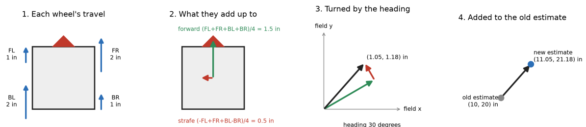
Figure 3.37. One loop of dead reckoning: the four wheel travels since the last loop, the forward and left arrows those add up to, the same pair turned to point along the robot's heading, and the old estimate with that pair added on the end.
