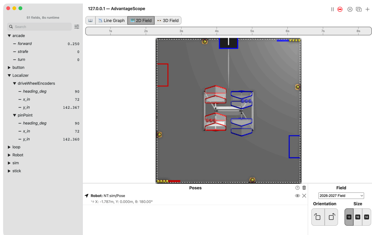
Figure 3.38. AdvantageScope's 2D Field with the robot at the top of the field, its arrow pointing up, and the list with the Localizer folder open: driveWheelEncoders/y_in climbs with pinPoint /y_in , and the two stay within a tenth of an inch.
