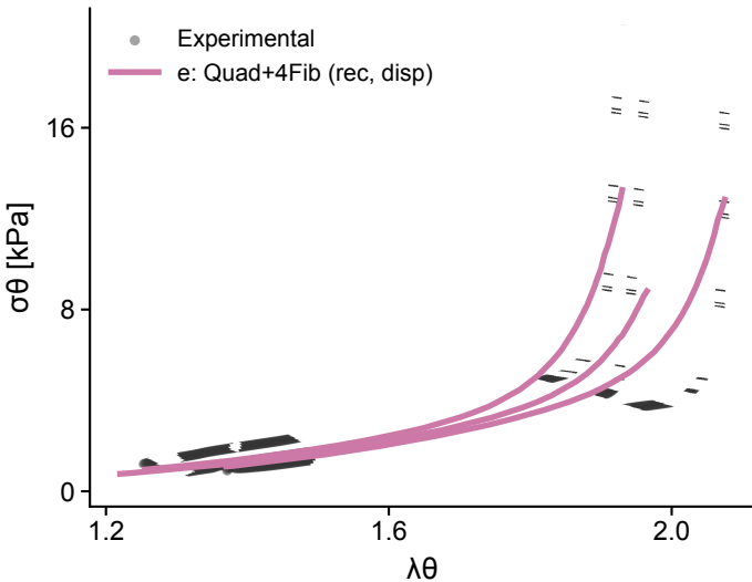
Variant E - Circumferential
