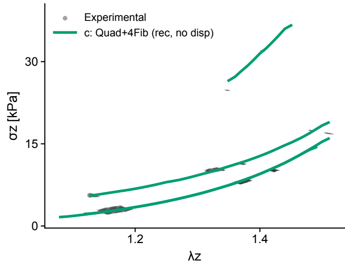
Variant C - Axial
