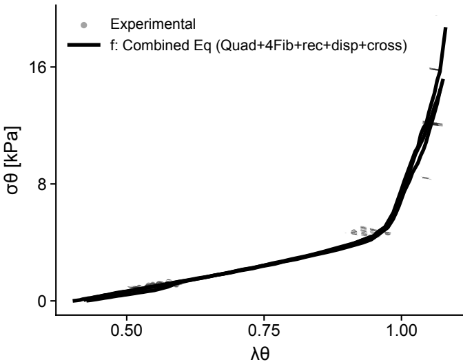
Variant F - Circumferential
