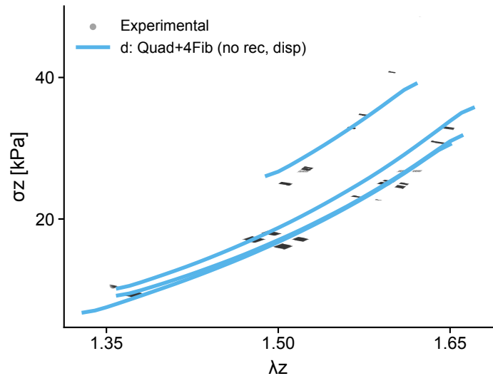
Variant D - Axial
