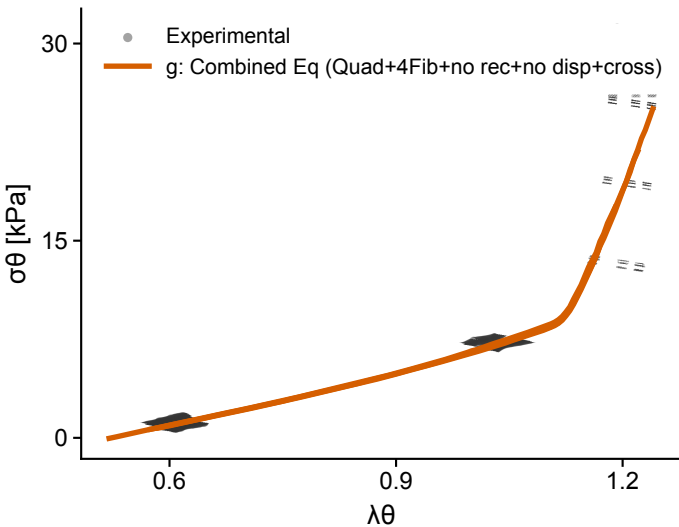
Variant G - Circumferential
